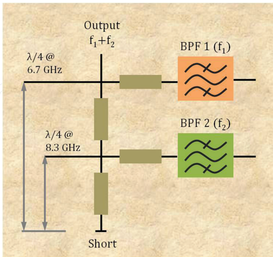
Figure 8. Frequency diplexer network [21].
