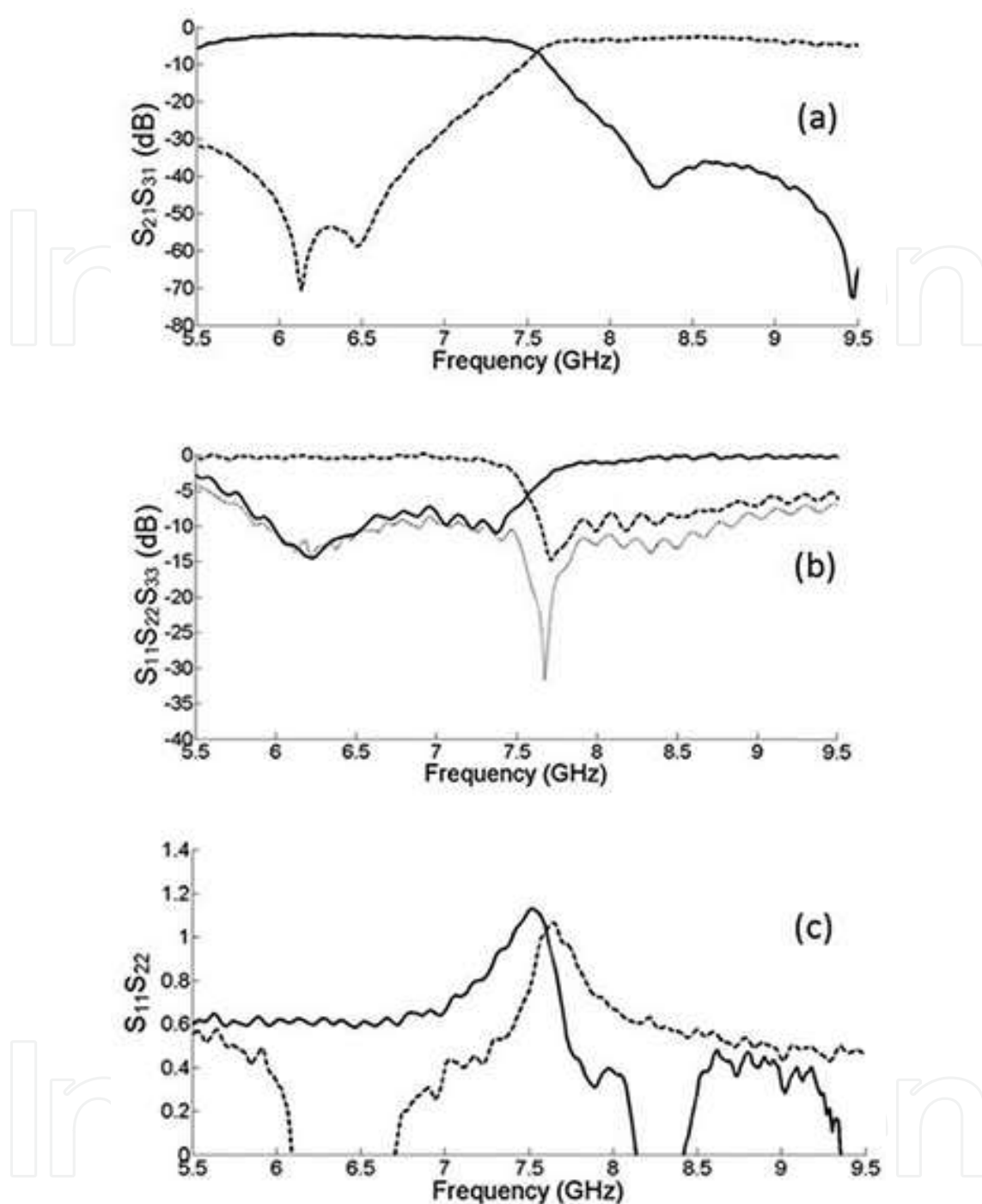
Figure 16. Measured results for FDN, (a) forward transmission, (b) input reflection, and (c) group delay.
