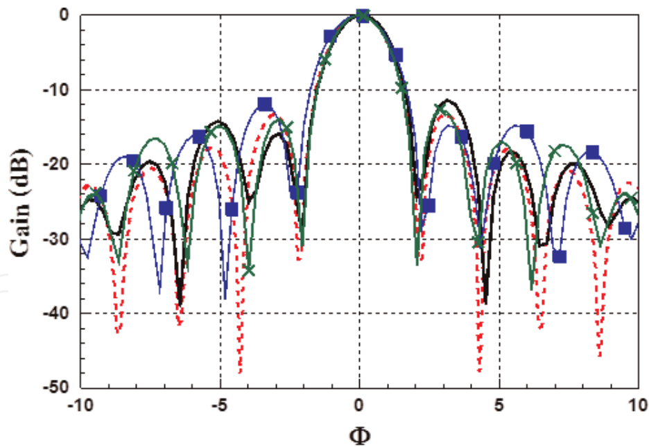
Figure 25. Radiation pattern of vertical polarized full array in azimuth plane ( \theta = 20^\circ cut). ( — Measured @ 11.9 GHz, - - - Simulated @ 11.9 GHz, —■— Measured @ 10.8 GHz, - - - Measured @ 12.8 GHz).
