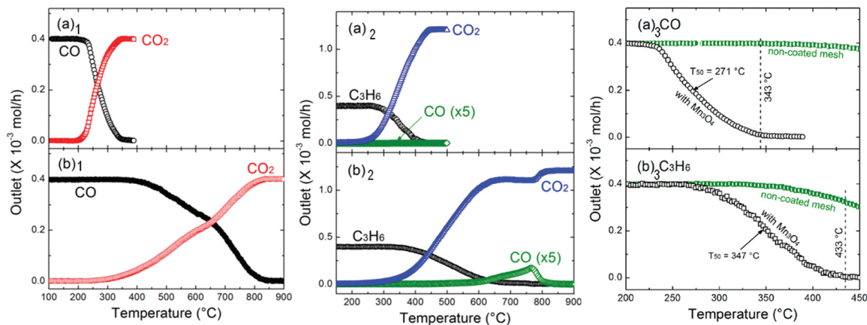
Figure 5. Production and light-off curves of CO and \text{C}_3\text{H}_6 oxidation over \text{Mn}_3\text{O}_4 -coated mesh ( a 1 , a 2 and a 3 ) and NCM ( b 1 , b 2 and b 3 ), respectively. Light-off curve of CO ( a 3 ) and \text{C}_3\text{H}_6 ( b 3 ) oxidation over \text{Mn}_3\text{O}_4 -coated mesh and NCM. The reaction was carried at the total flow rate was kept at 15 \text{ ml min}^{-1} with 1% of \text{C}_3\text{H}_6 and 10% of \text{O}_2 diluted in Ar corresponding the WHSV of 45,000 \text{ g}_{\text{cat}}^{-1} \text{ h}^{-1} . Reproduced with permission from [43]. Copyright 2013, American Chemical Society.
