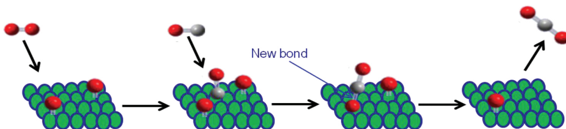
Scheme 2. Schematic illustration of the LH process for CO oxidation.
