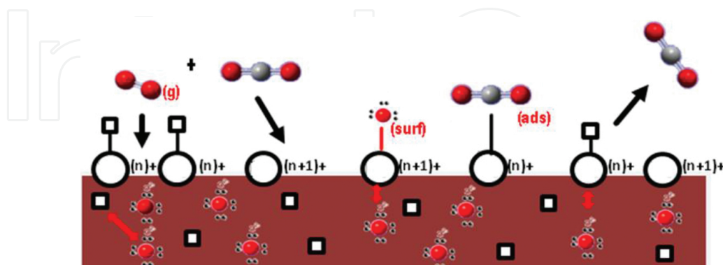
Scheme 3. Illustration of the MvK mechanism for CO oxidation.
