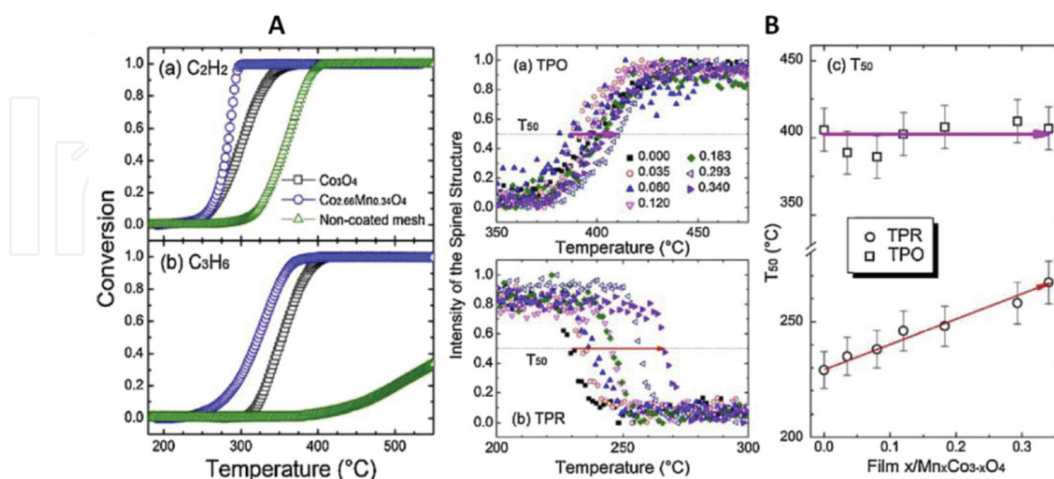
Figure 10. (A) Light-off curves of C_2H_2 and C_3H_6 over Co_{3-x}Mn_xO_4 ( x=0 and 0.34 ) spinel structures grown on mesh of stainless steel substrates and NCM. The reaction was carried at the total flow rate was kept at 15 \text{ ml min}^{-1} with 2% of fuel and 20% O_2 diluted in Ar at a total flow rate of 0.015 \text{ L/min} ; (B) TPO/TPR patterns of Co-Mn oxide. Reproduced with permission from [45]. Copyright 2015, Elsevier.
