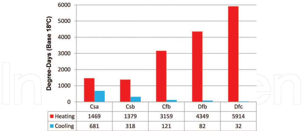
Figure 7. Average annual heating and cooling degree-days for five climatic regions [1].
