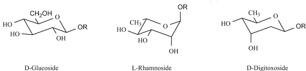
Figure 3. Examples of sugar residues attached to cardenolides.
