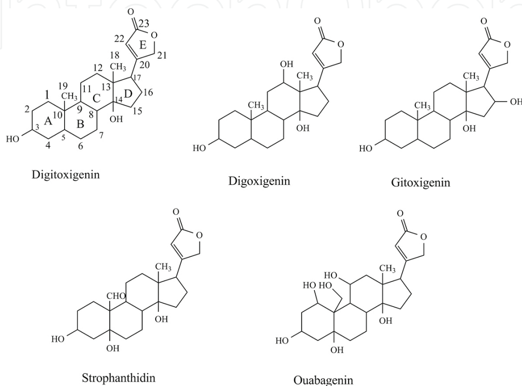
Figure 2. Structures of some common cardiac aglycones.
