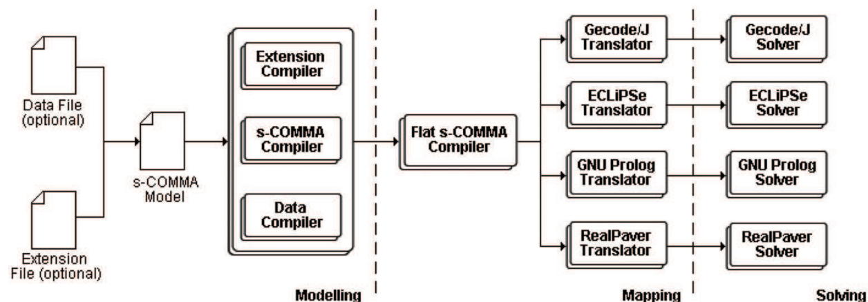
Fig. 7. s-COMMA architecture.
