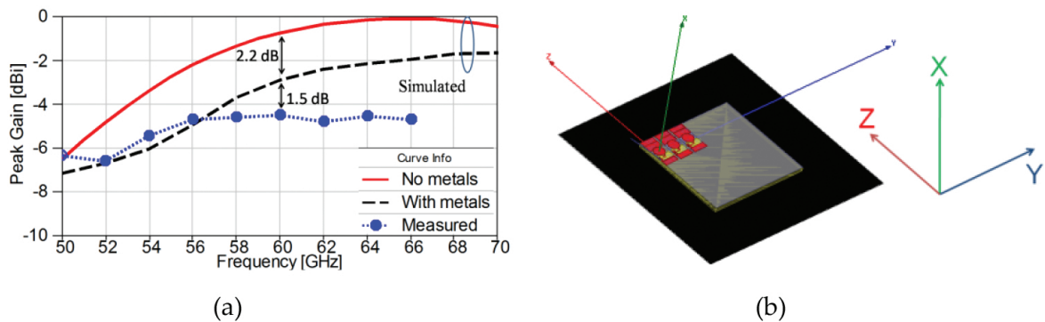
Figure 11. (a) Measurement results using the setup in Ref. [25]. (b) HFSS model for measurement validation. “Reprinted with permission from Microwave Journal.”
