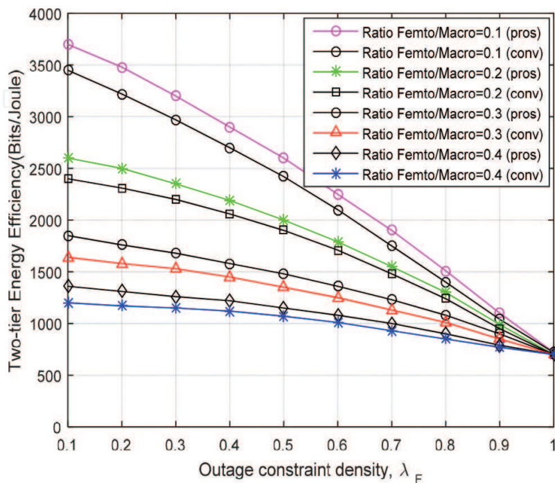
Figure 7. Two-tier network energy efficiency versus density.
