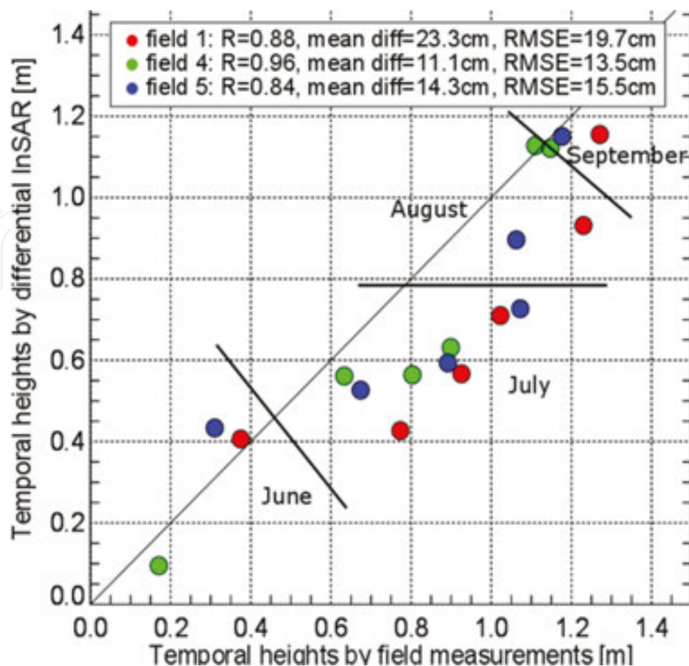
Figure 10. Comparison between interferometric height and ground truth in form of scatterplot for three fields.
