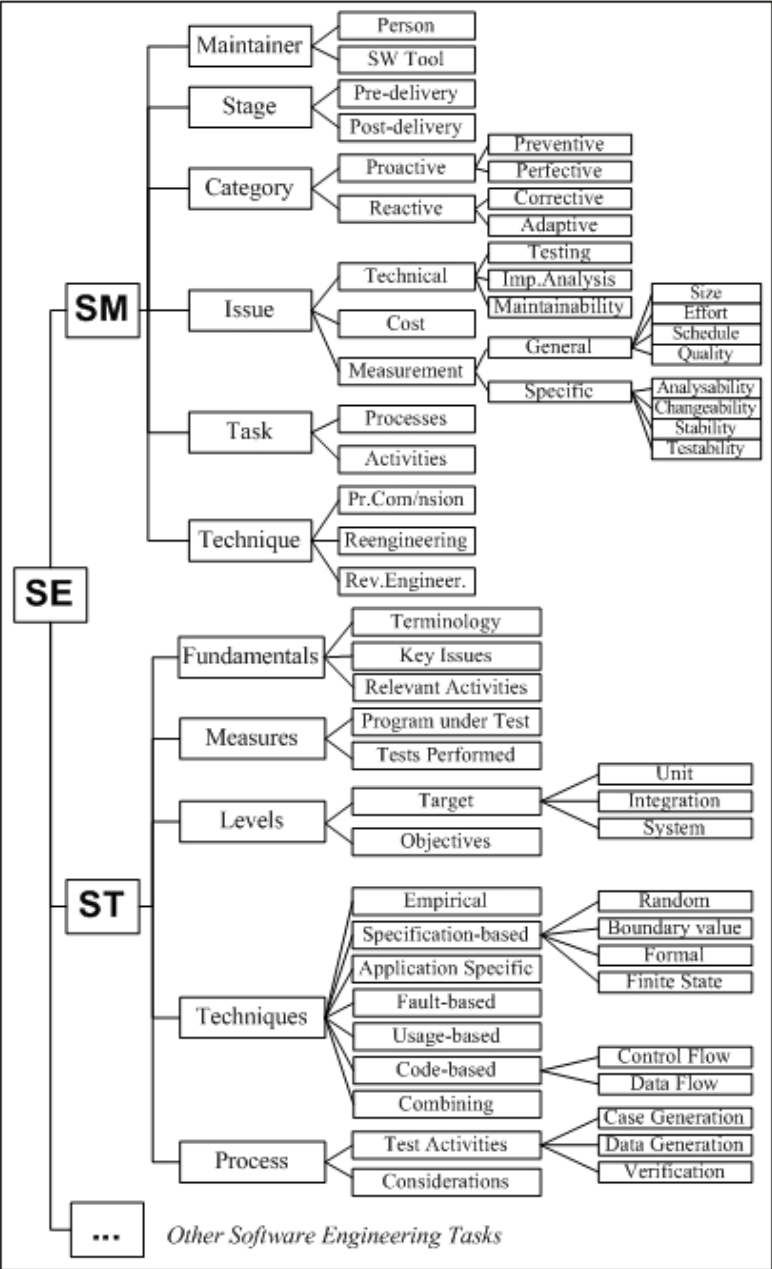
Fig. 3. Software Engineering (SE) Taxonomy
