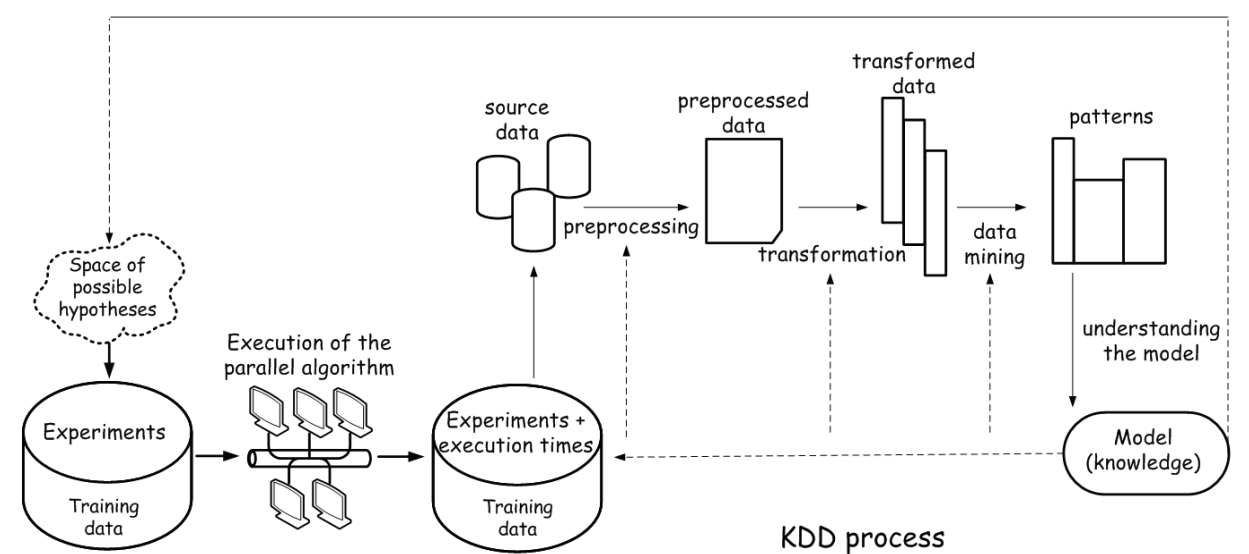
Figure 3. The knowledge construction model
