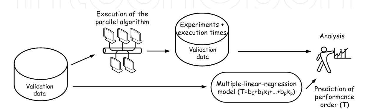
Figure 4. The validation of the model
