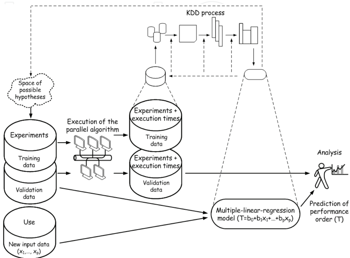
Figure 2. The performance prediction methodology
