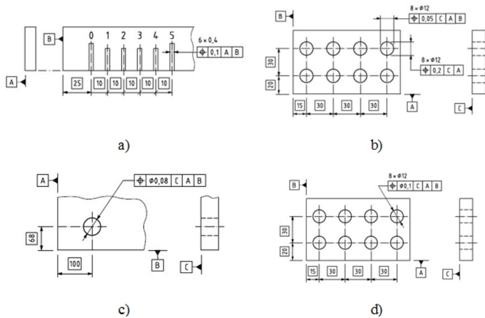
Figure 6. Position tolerance of a line.
