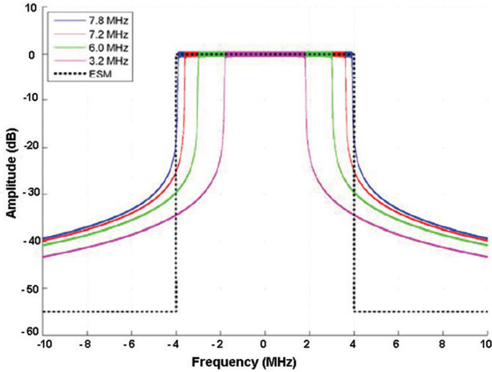
Figure 1. Power spectral density of CP-OFDM centred on the active carrier [9].
