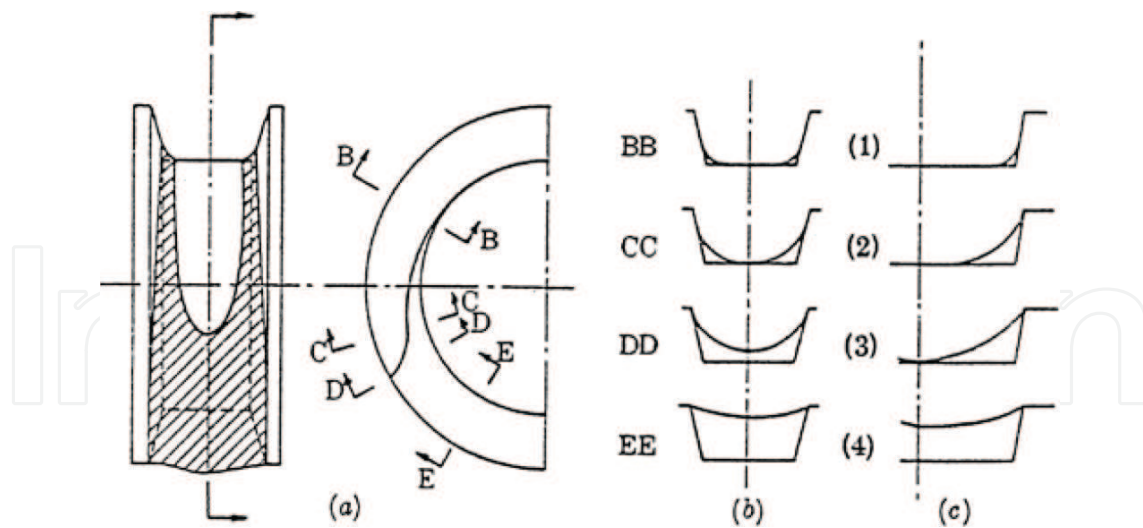
Figure 3. Configuration of retained liquid or condensate around a horizontal integral-fin tube. (a) Condensate retention on integral-fin tube. (b) Configuration of liquid around the narrow-spaced integral-fin tube. (c) Configuration of liquid around the wide-spaced integral-fin tube (after Masuda and Rose [15]).
