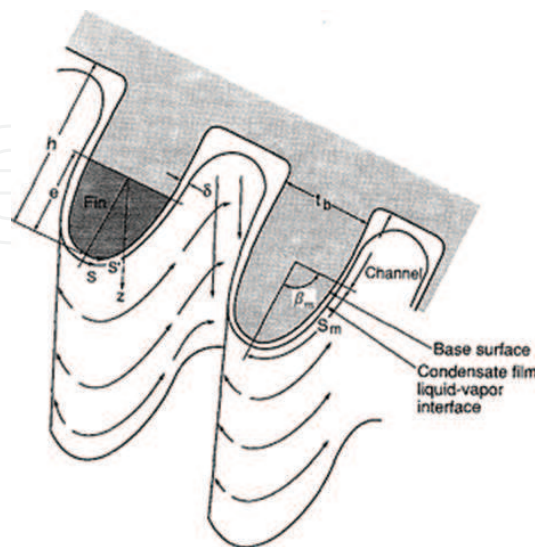
Figure 6. Fin parameters of vertical-fluted tube (after Gregorig [51]).
