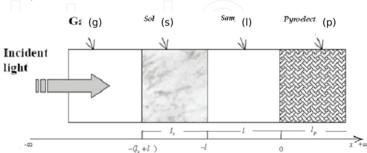
Figure 2. 1D configuration of TWC showed that the thermal waves are partially reflected and transmitted upon striking the boundaries (g, s, l, p and b) which stand for gas, solid, liquid sample, PVDF film and backing, respectively.
