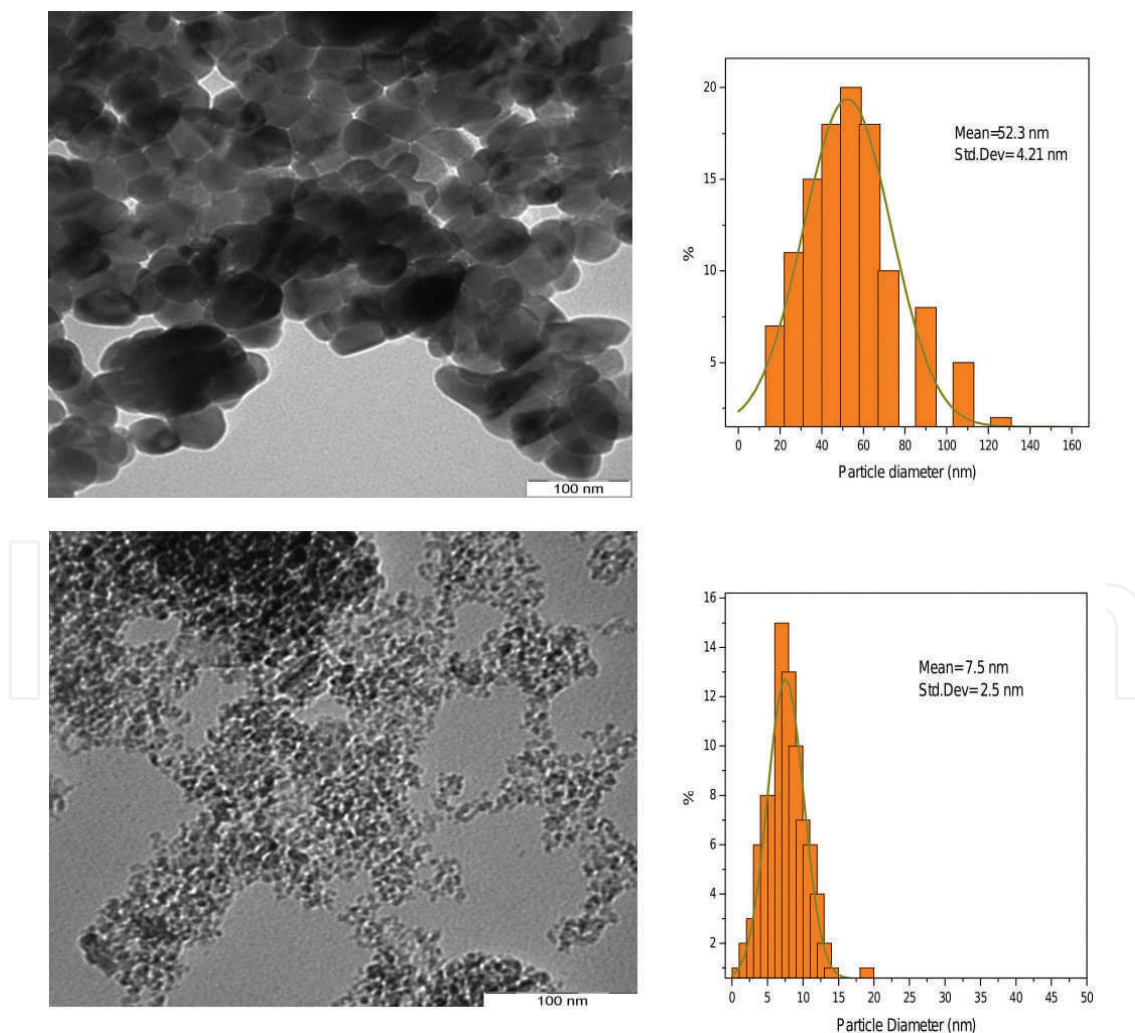
Figure 14. TEM images and their size distributions of (a) CuO particles and (b) \text{Al}_2\text{O}_3 nanofluids prepared in water [56].
