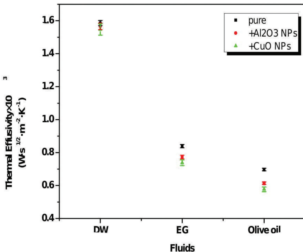
Figure 16. Thermal effusivity of \text{Al}_2\text{O}_3 and \text{CuO} nanofluids with (DW, EG and olive oil) and their pure solvents [56].
