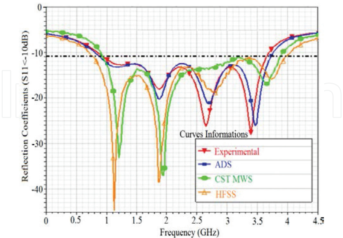
Figure 2. Simulated and measured reflection coefficients of the proposed LWA.
