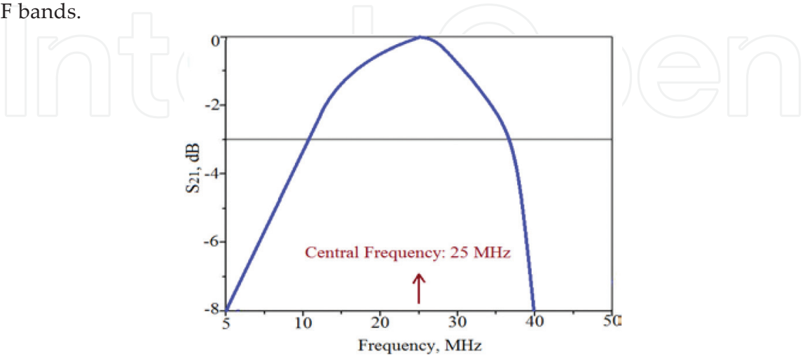
Figure 17. Impedance-matching LC circuit response.
