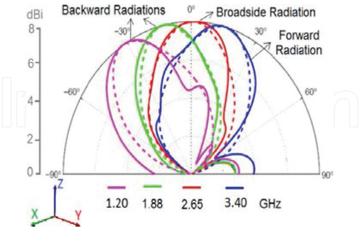
Figure 3. 2-D radiation patterns in dB scale at spot frequencies. Solid lines: measured results and dashed lines: simulated results.
