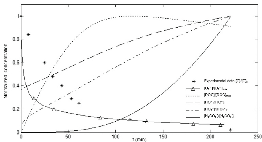
Figure 5. Concentration-time profiles of \text{HO}^\bullet (---), \text{HO}_2^\bullet (-.-.-), \text{O}_2^{\bullet-} (-Δ-), DOC (···) and \text{H}_2\text{CO}_3^* (—) using the prediction kinetic model A. (*) represents PHE experimental evolution. Operating conditions: \text{H}_2\text{O}_2/\text{PHE} = 495 ; [\text{C}]_0 = 2.23 \times 10^{-3} \text{ M} ; t = 220 \text{ min} .
