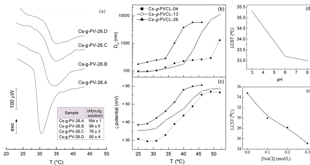
Figure 4. (a) Heating \mu DSC scans of 10 wt% aqueous solutions of Cs-g-PV-26.A, Cs-g-PV-26.B, Cs-g-PV-26.C and Cs-g-PV-26.D samples (heating rate, 0.6 °C min -1 ; reference, water). Reprinted from Ref. [85]. Copyright 2015, with permission from Elsevier. Dependence of the (b) hydrodynamic diameter, D_{Hr} and (c) \zeta -potential of Cs-g-PVCL on temperature of aqueous solutions of Cs-g-PVCL for different number-average molecular weights of PVCL-grafted chains. Cs-g-PVCL samples with Mn 04, 13, and 26 kDa at 2 mg mL -1 (pH 6). Heating rate, 0.25 °C min -1 . Variation of LCST of the Cs-g-PVCL-26 solution (2 mg mL -1 ) with (d) pH of the medium and (e) ionic strength. Heating rate, 0.25 °C min -1 . Reprinted from Ref. [96]. Copyright 2016, with permission from Springer.
