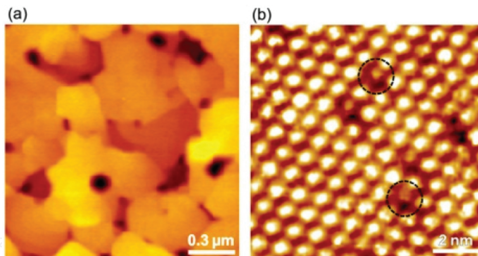
Figure 23. (a) AFM image ( 1.5 \times 1.5 \mu m^2 ) and (b) high-resolution STM image ( 10 \times 10 nm^2 ) of C_{60} -deposited Au/mica surface. Note that STM image was obtained under electrochemical condition in 0.1 M HClO_4 .
