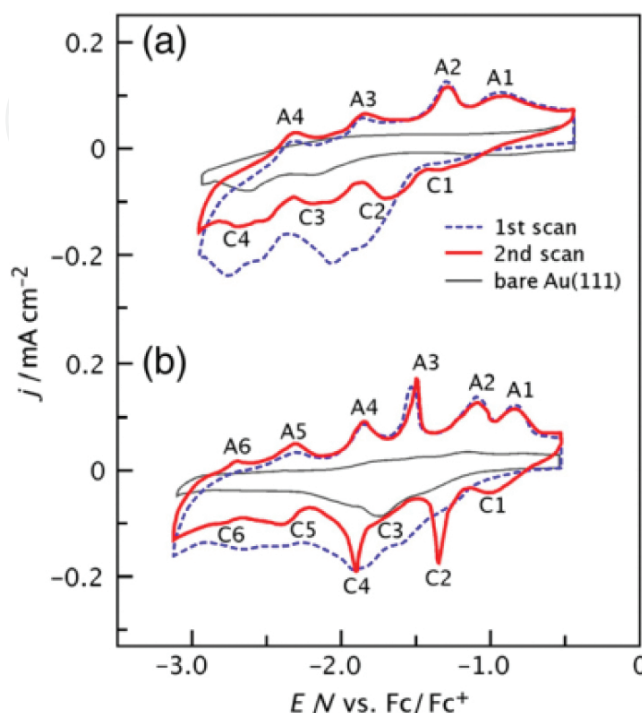
Figure 26. Typical cyclic voltammograms of a clean Au(1 1 1) electrode (gray line) and a C_{60} -modified Au(1 1 1) electrode obtained in [TFSI] - -based ILs with (a) [N_{1,4,4,4}]^+ and (b) [C_4mpyr]^+ , respectively, at 25 °C. The blue dotted and red solid lines indicate the first and second scans, respectively, of the C_{60} -modified Au(1 1 1) single-crystal electrode. The scan rate was 0.5 V s -1 .
