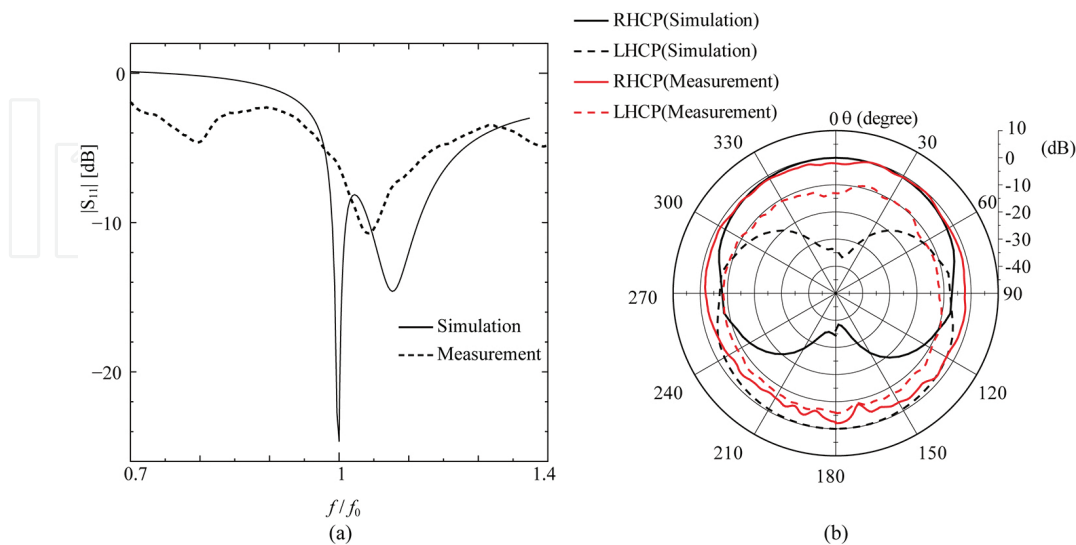
Figure 13. Characteristics of the CSA prototype as shown in Figure 12 : (a) S11 characteristics, and (b) radiation patterns at f = f_0 and \phi = 0^\circ .
