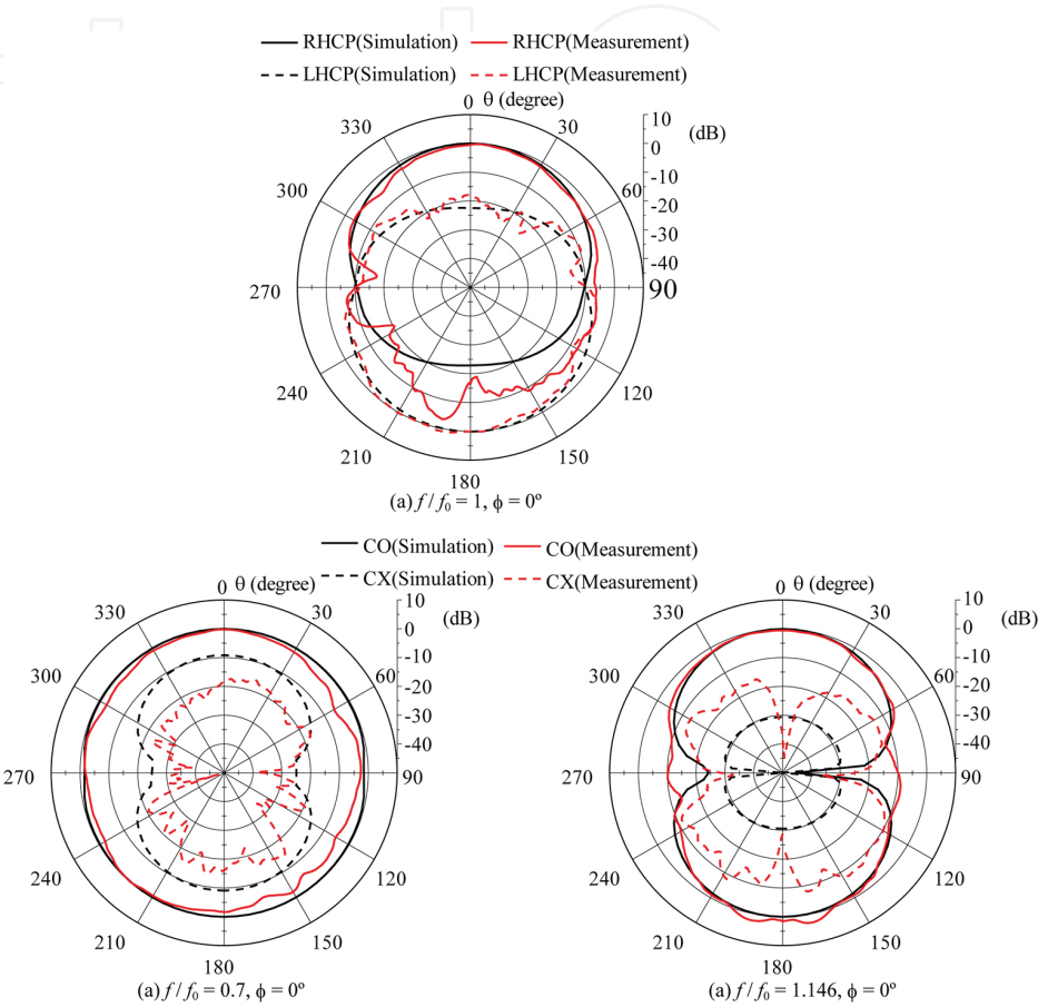
Figure 16. Radiation patterns at three resonant frequencies.
