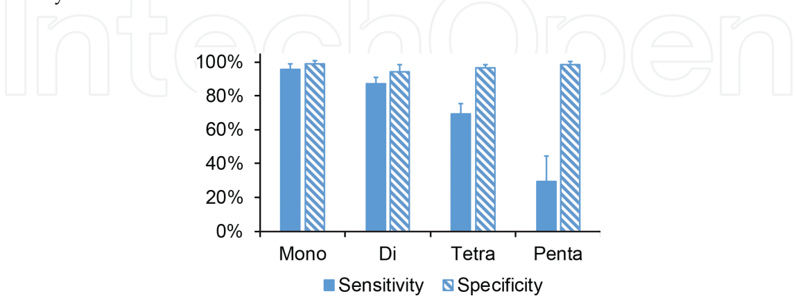
Figure 2. The relative sensitivity and specificity of mono-, di-, tetra- and penta-nucleotide repeats for detection of MSI in mismatch repair deficient CRC.
