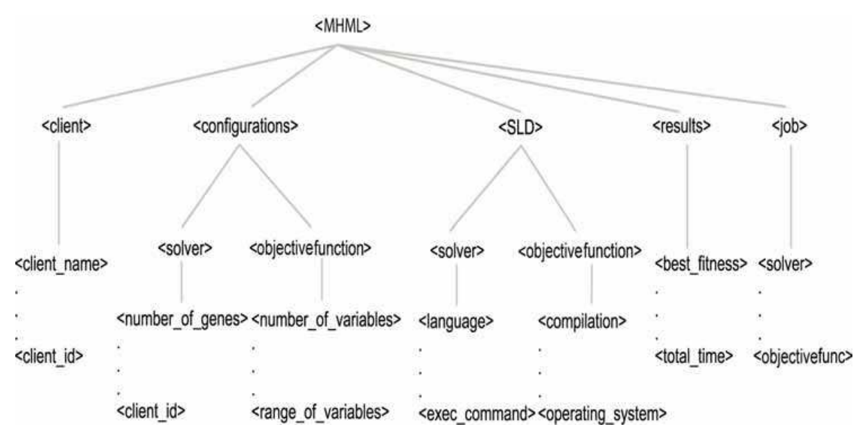
Fig.8.Top level hierarchy of MHML.
