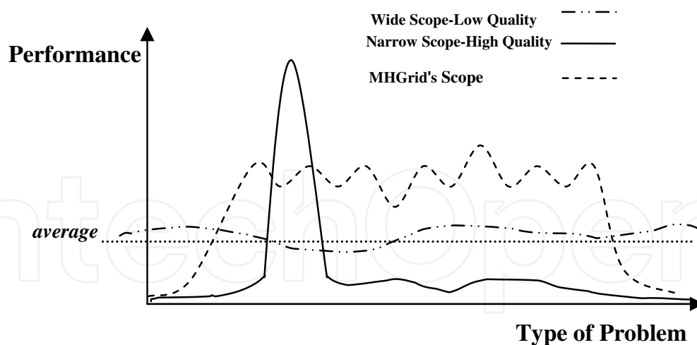
Fig.9. MHGrid scope according to problem-type space.
