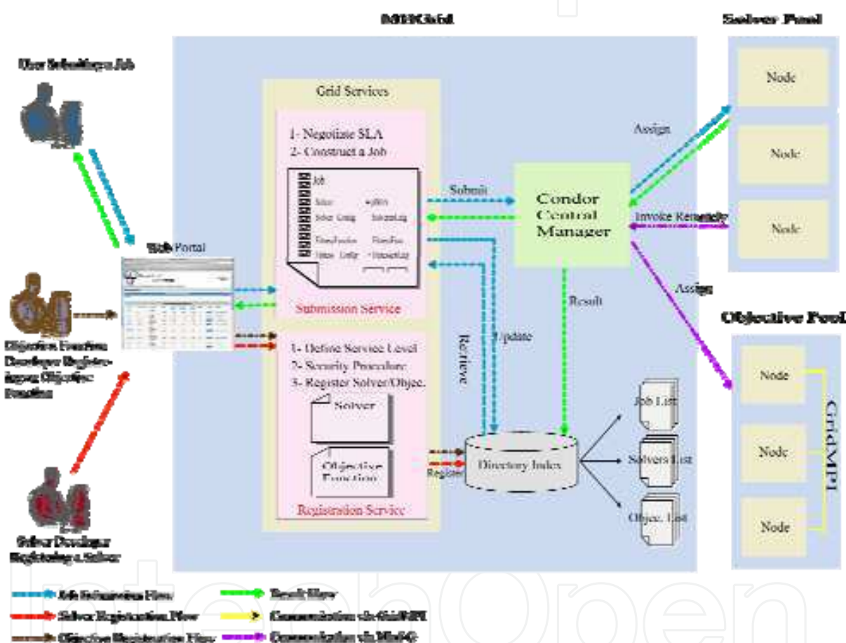
Fig.4. A close-up to MHGrid internals.
