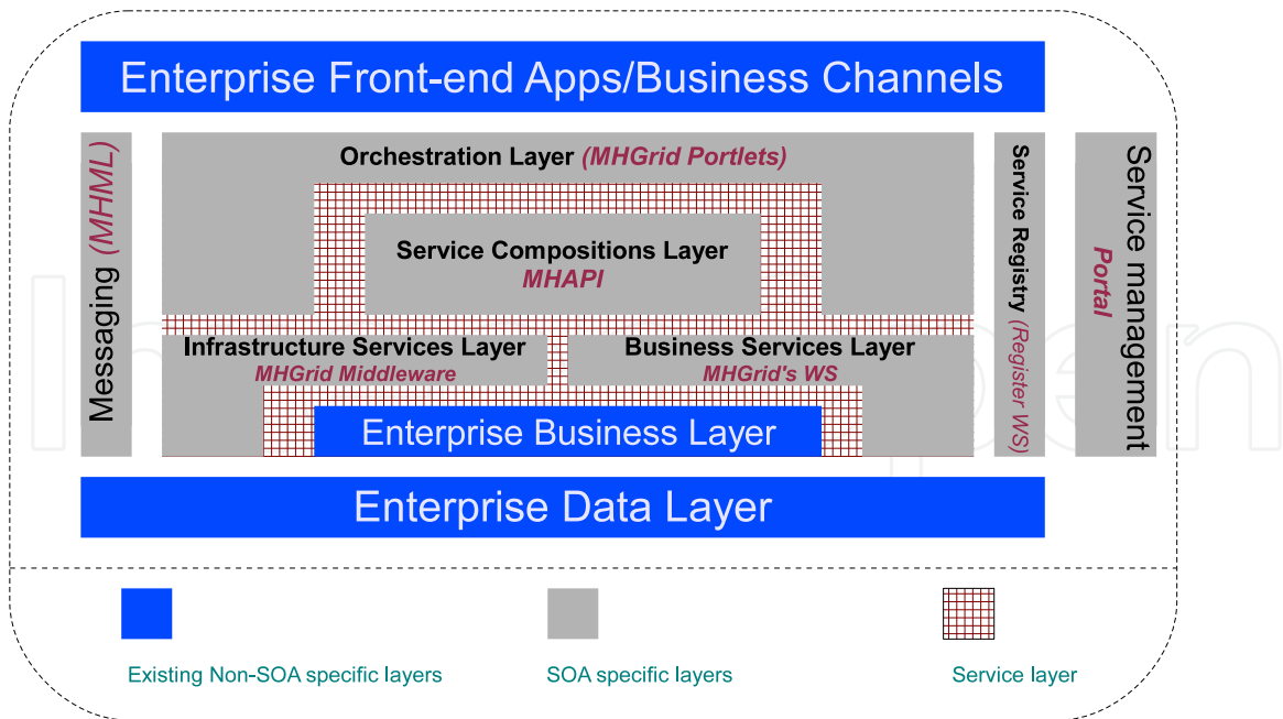
Fig.10. MHGrid modules mapped to a typical SOA layout.
