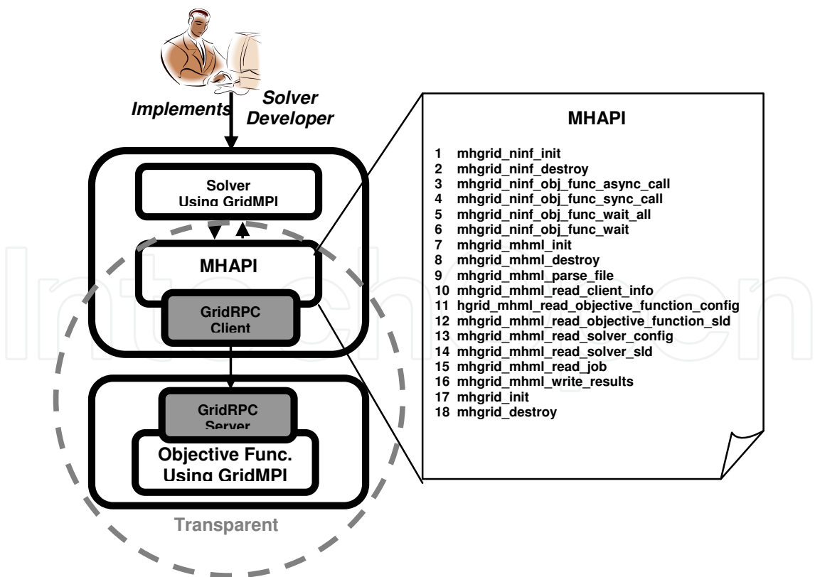
Fig.6.Main functionalities provided by MHAPI. Note that every thing is kept transparent from the solver developer.
