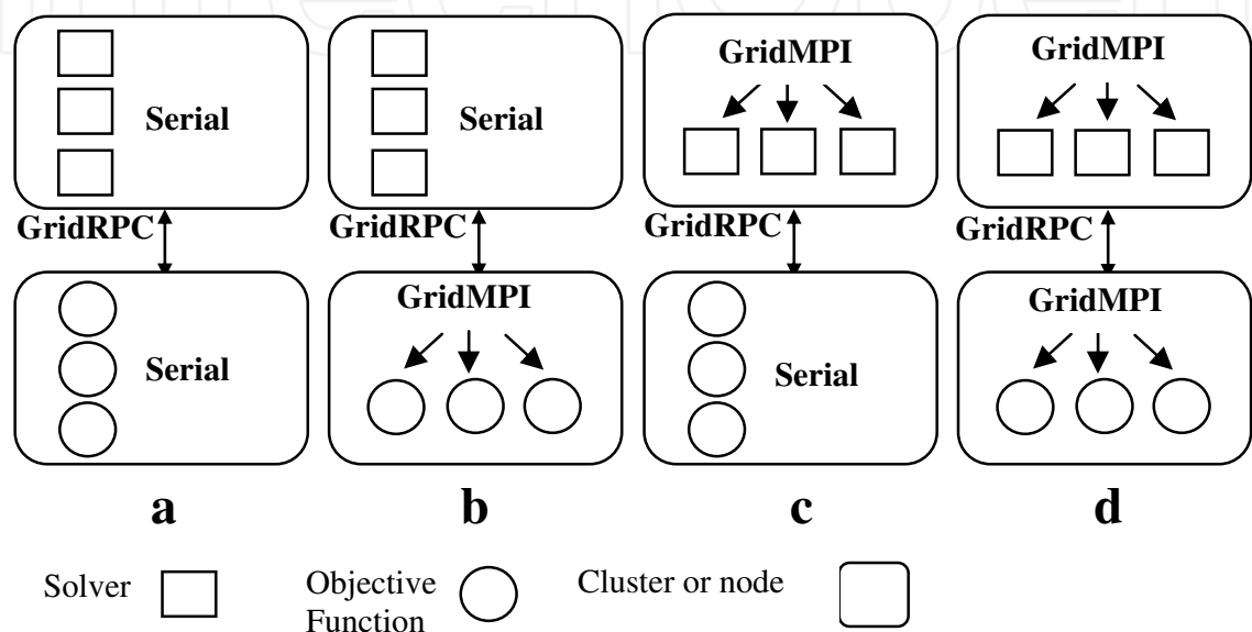
Fig. 5.Different grain size depending on parallelization combination. a) A solver running in serial fashion and objective function computing also running in serial, simplest scenario with no parallelization. b) The solver running serial but the objective computing is running parallel in another cluster, Master-slave GAs are an example that will use this scenario. The Master here is the solver process running in serial and the GridMPI objective function processes are the slaves. c) The solver running in parallel while objective function calculation is serial, a solver like parallel BOA will use this scenario where the objective function calculation is not heavy while the solver involves heavy computation (candidate selection). In this scenario one of the GridMPI solver processes is a controlling node that will call upon objective function calculation. d) Both solver and objective function are running in parallel on different clusters. This scenario will have one of the GridMPI solver processes acting as a controlling node that will be acting as a master for the GridMPI objective function processes.
