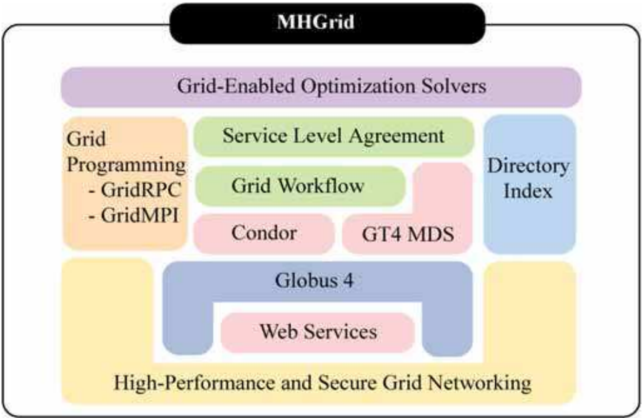
Fig.3. MHGrid architecture at an abstract level.
