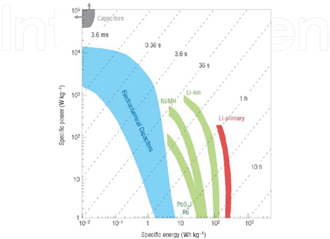
Figure 1. Specific power and energy for various electrical energy storage devices show in Ragone plot [4].
