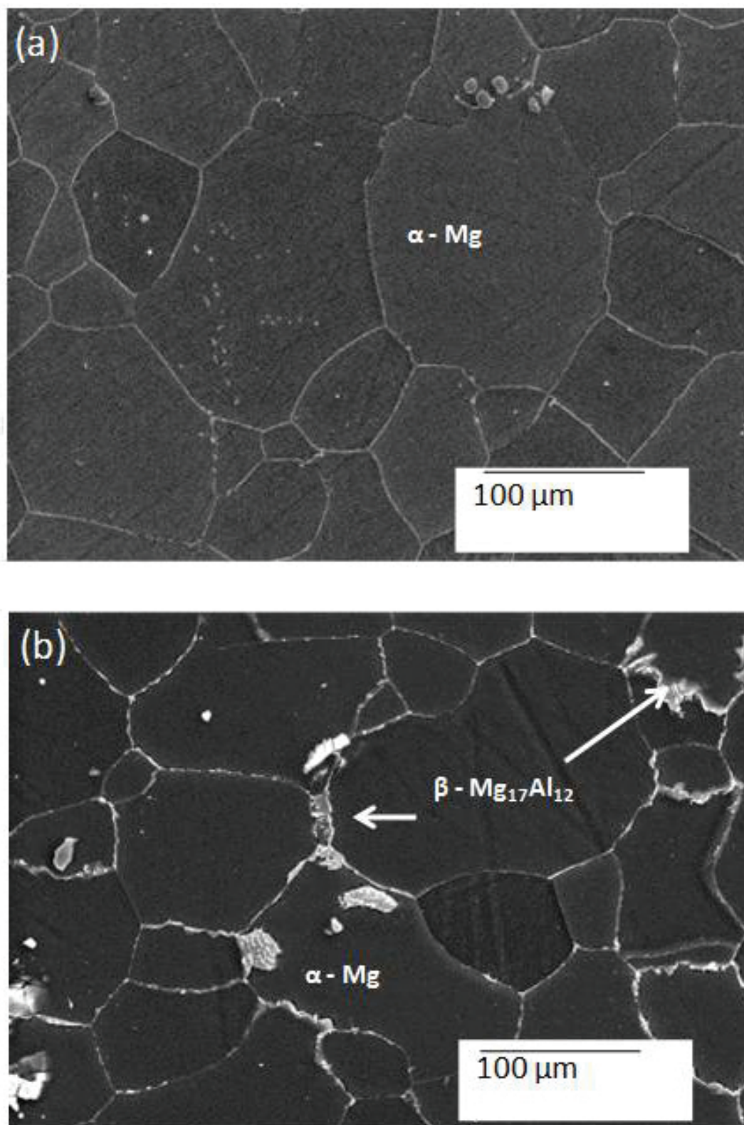
Figure 7. (a) SEM micrographs of AZ31 and (b) AZ61 magnesium alloys.
