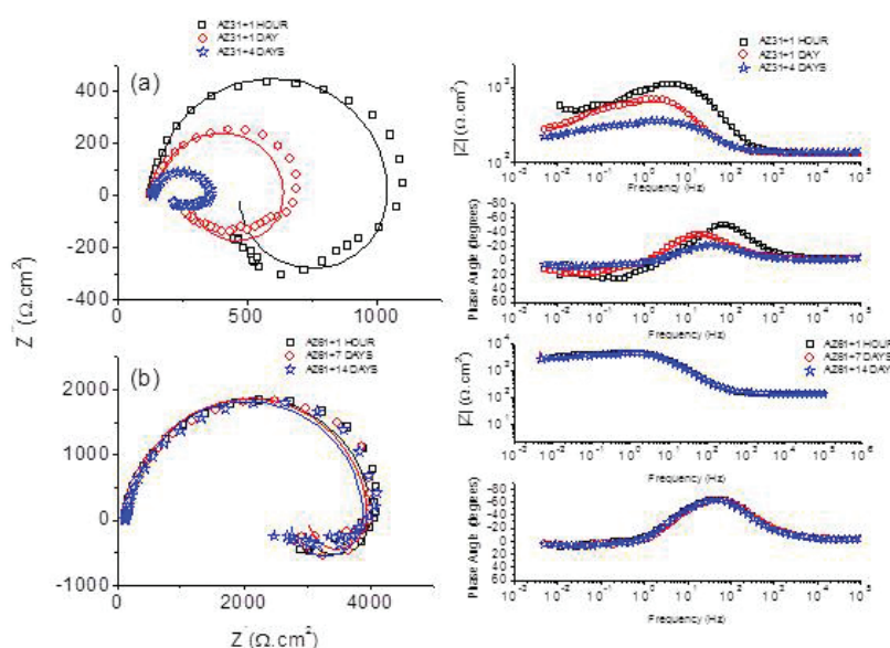
Figure 5. Example of Nyquist and Bode plots with respective fitting for AZ31 and AZ61 alloys with different immersion times in 0.6 M NaCl solution.
