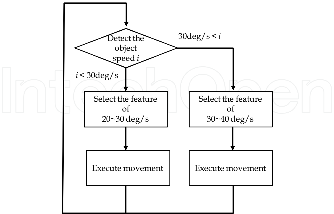
Fig. 11. Implementation model
