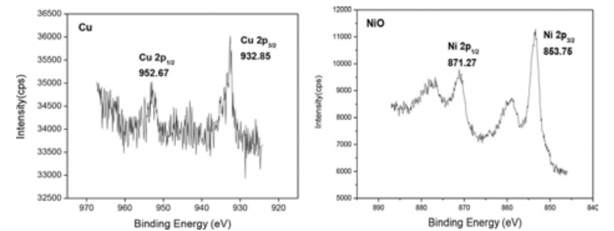
Figure 30. XPS spectra of Cu 2p, Ni 2p in Cu@Ni nanoparticles.
