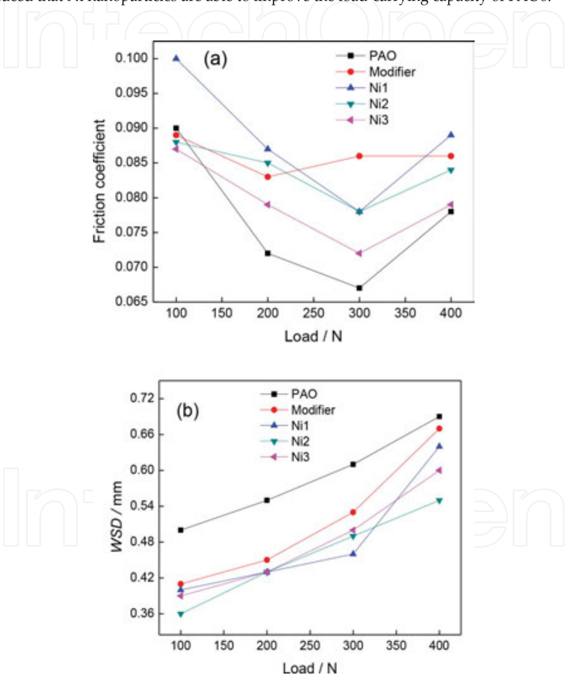
Figure 8. Friction coefficient (a) and wear scar diameter (b) versus applied load under the lubrication of PAO6, PAO6 + surface-modifiers, and nanolubricants containing 0.05% Ni nanoparticles with different size (four-ball friction and wear tester, 1450 rpm, 30 minutes).
