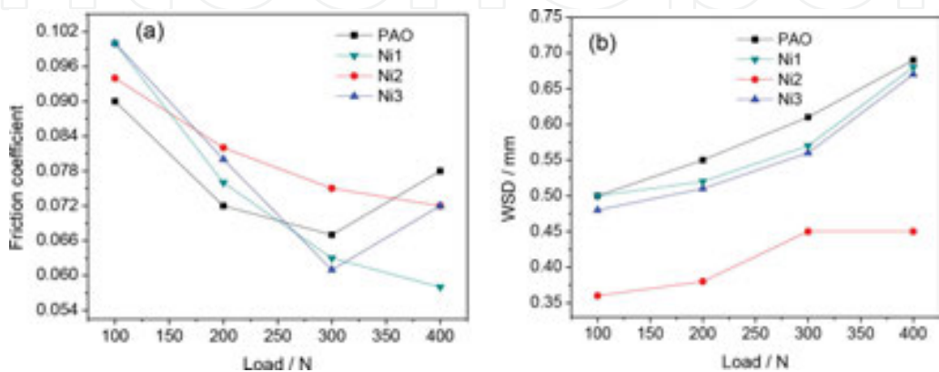
Figure 16. Friction coefficient (a) and wear scar diameter (b) versus applied load under the lubrication of PAO6 and 0.2% Ni nanoparticles with different morphology (four-ball friction and wear tester, 1450 rpm, 30 minutes).
