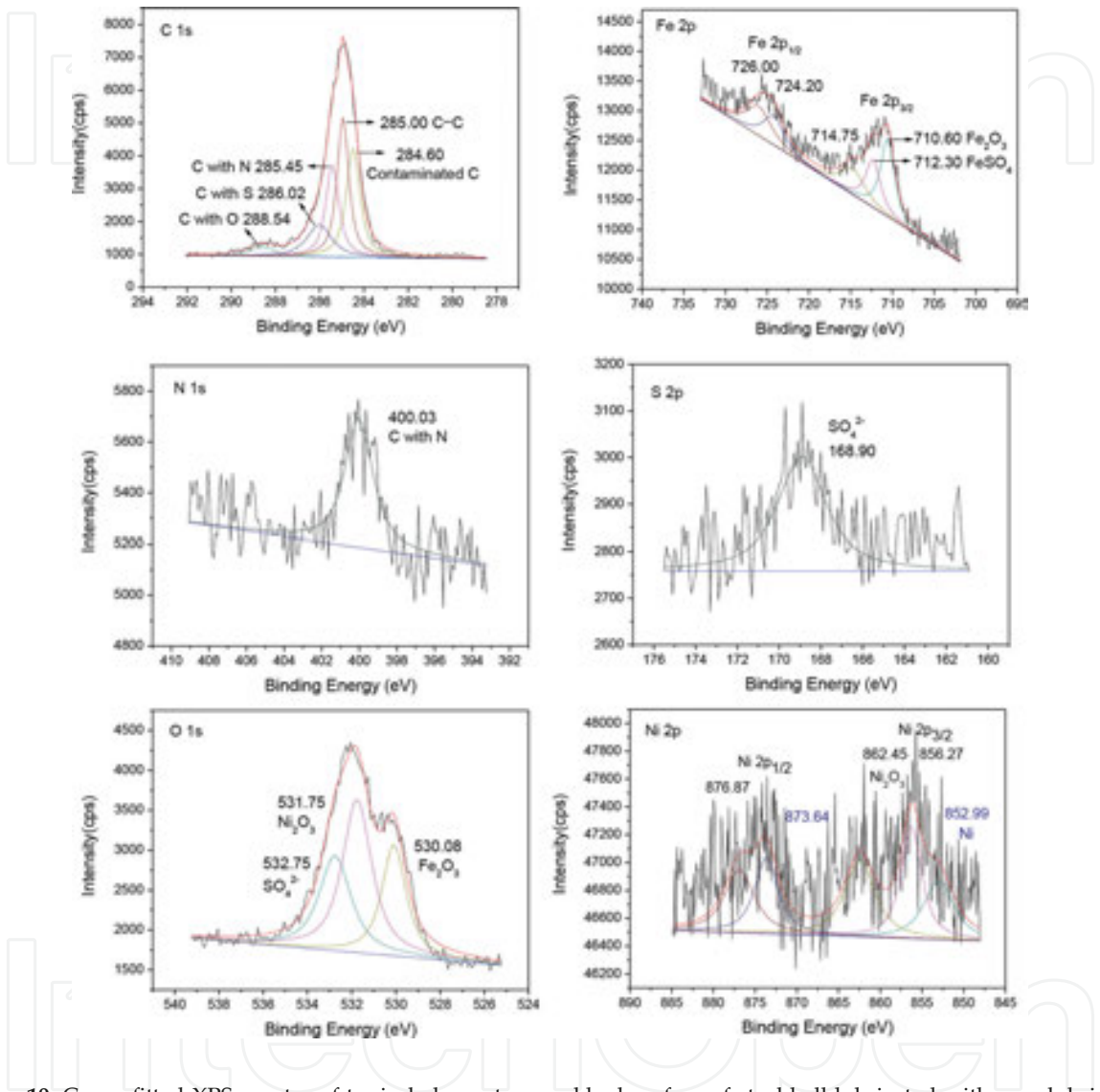
Figure 19. Curve-fitted XPS spectra of typical elements on rubbed surface of steel ball lubricated with nanolubricants containing 0.2% Ni (four-ball friction and wear tester, 1450 rpm, 400 N, 30 minutes).
