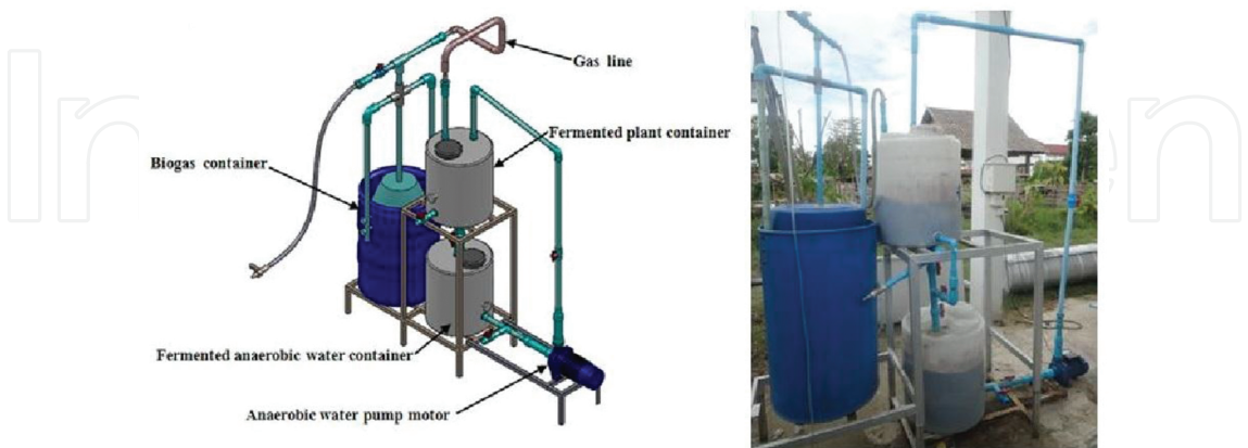
Figure 4. Dry fermentation anaerobic digestion process.
