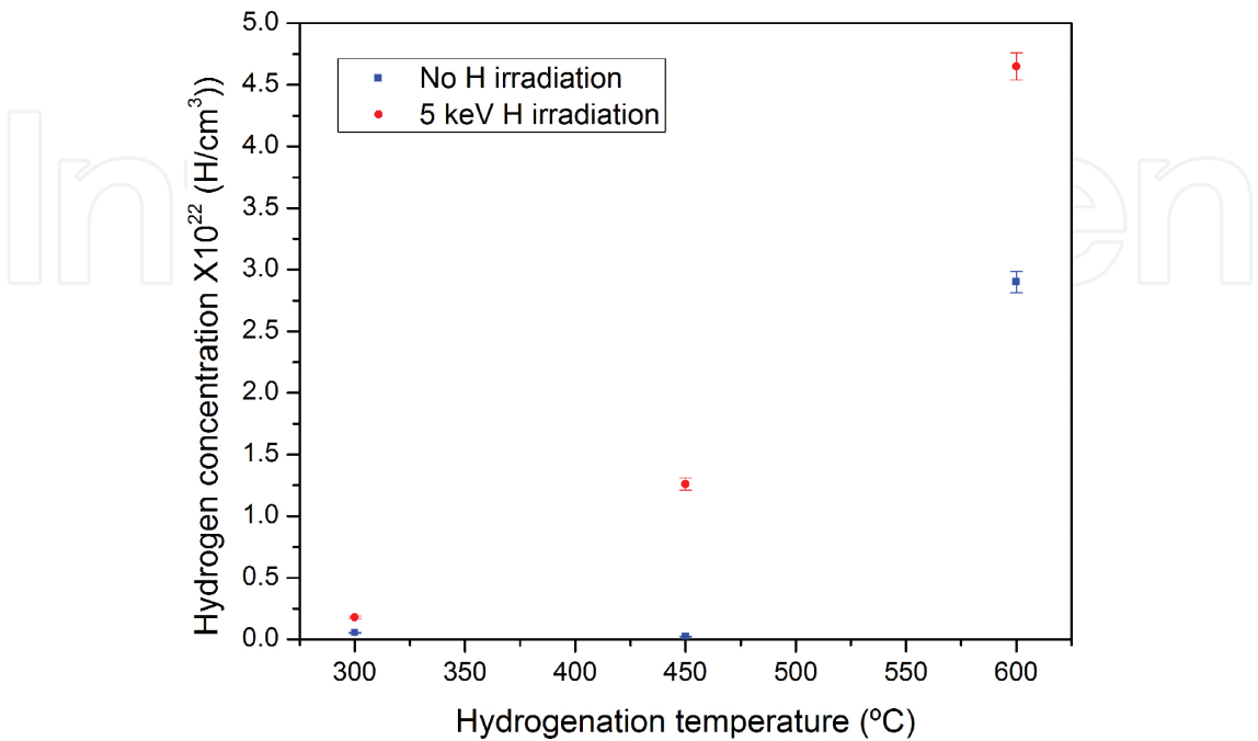
Figure 7. Hydrogen concentration of the hydrogenated samples, before and after implantation [13].
