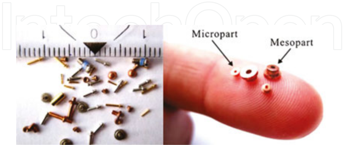
Figure 2. Mechanical microparts formed by microforming [7, 8].
