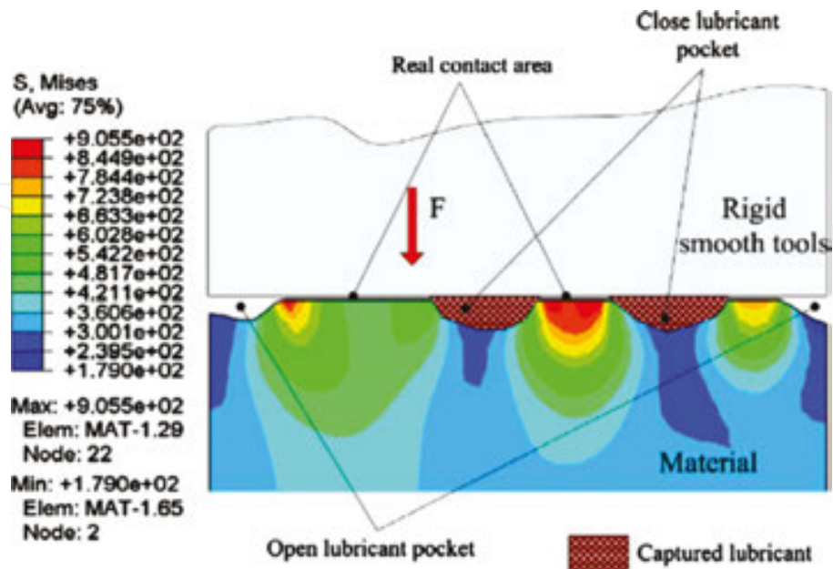
Figure 26. 2D sketch of OLPs, RCAs, and CLPs [32].
