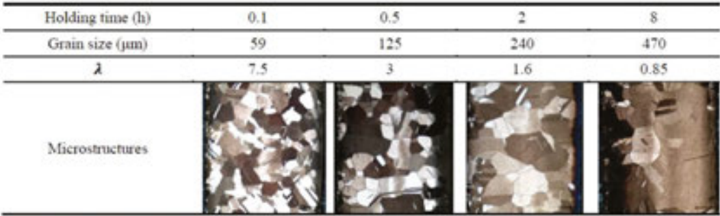
Figure 17. Microstructure of specimens and grain size, \lambda = specimen radius/grain size [25].
