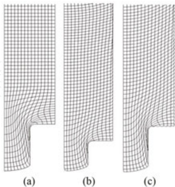
Figure 32. Flow nets of microextruded metal rods with a tool surface characterized by: (a) constant friction factor; (b) and (c) rigid triangular waves [39].
