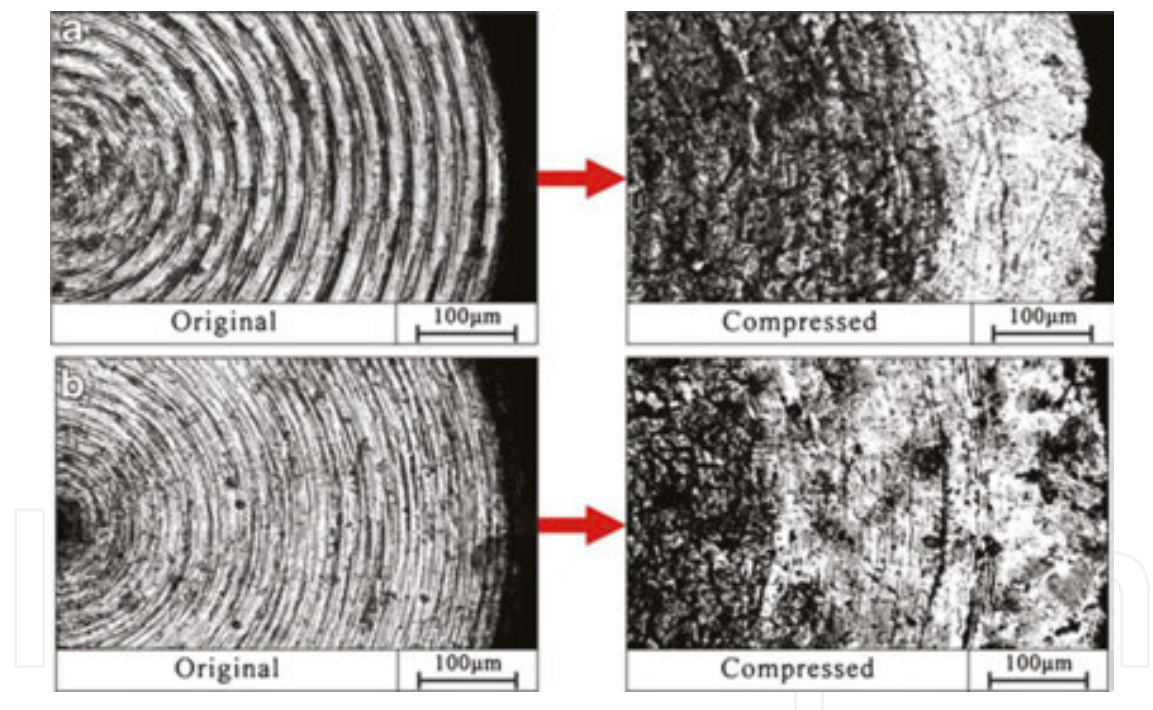
Figure 28. End surface topographies of the specimens ( \varnothing 1 \times 1.5 mm) with the asperity size of: (a) 25 µm; and (b) 10 µm [32].
