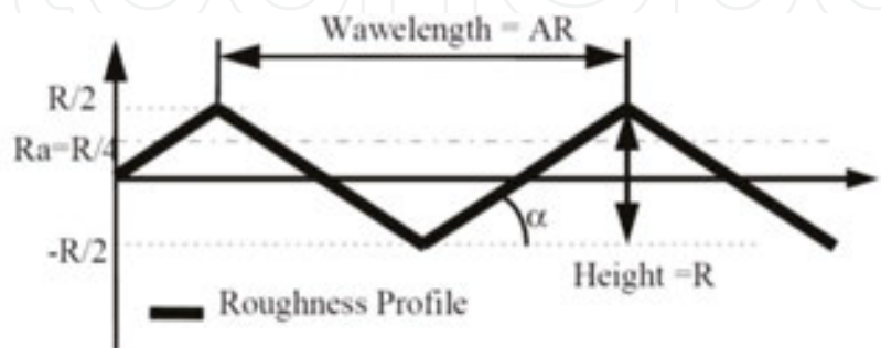
Figure 31. Triangular wave surface roughness model [36].
