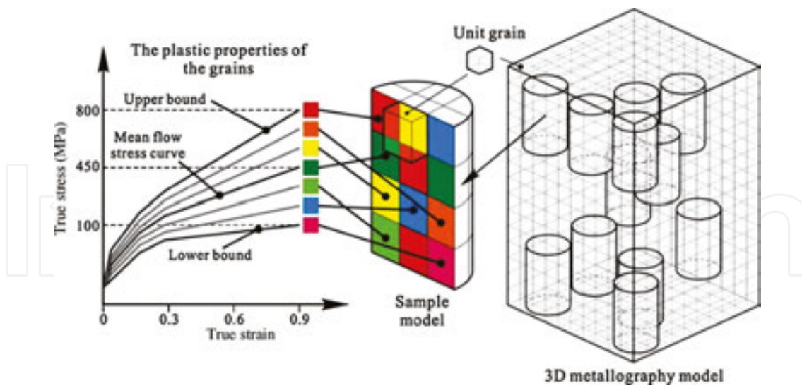
Figure 14. Schematic illustration of the 3D full-scale model with cubic grain.
