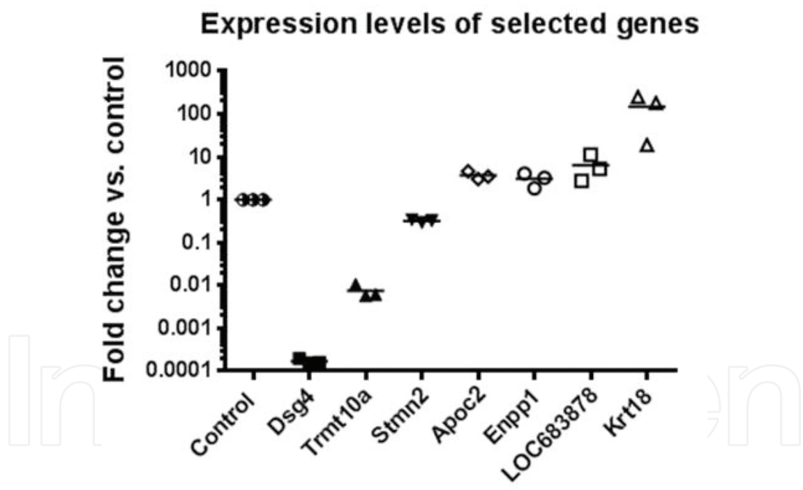
Figure 5. Changes in mRNA expression after recultivation in vitro: ASML cells were also recultivated in vitro for 3, 6, and 9 days after they had been reisolated from rat liver after a colonization period for 21 days. As a result, some genes were downregulated or upregulated in vitro, at varying degrees. Seven examples are given in comparison to control.
