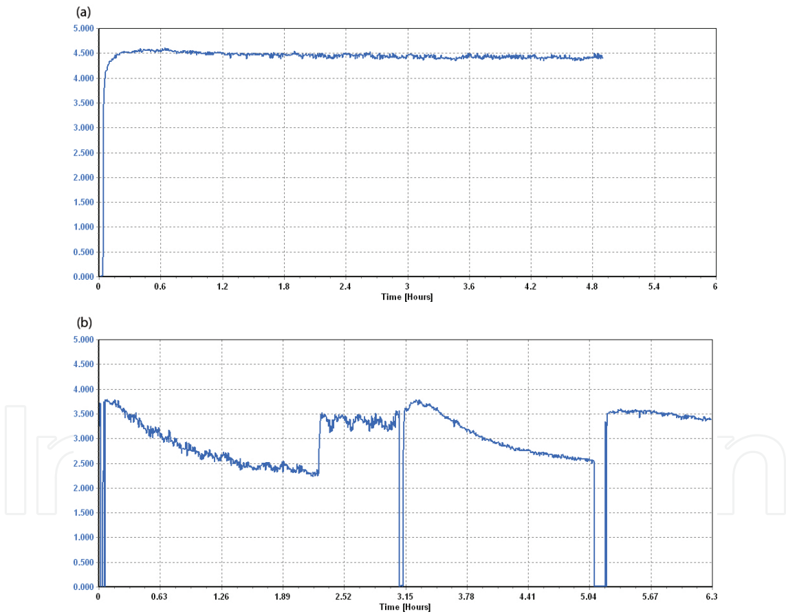
Figure 8. Second harmonic generator output power versus time using thermo stabilized compressor module (a) and nonstabilized one (b).
