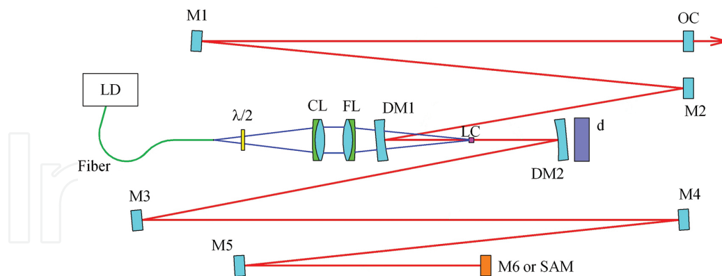
Figure 2. Schematic diagram of the Yb:KYW laser pumped by laser diode (LD) [25]. \lambda/2 – half wave plate; CL – collimating lens; FL – focusing lens; LC – Yb:KYW laser crystal; DM1, DM2 – spherical dichroic mirror; M1–M6 – cavity mirrors; OC – output coupler; SAM – semiconductor saturable-absorber mirror; d – dumper for blocking and cooling.
