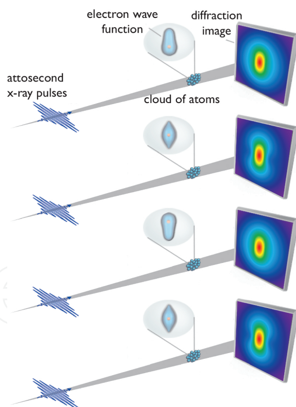
Figure 8. Attosecond X-ray diffraction: as a coherently induced charge oscillation takes place in an atom or molecule, an incident X-ray pulse takes a diffraction snapshot of the electron distribution at the time of interaction; changing the time delay between the source of the excitation and the attosecond pulse allows for the temporal evolution of the charge density to be directly measured in time and space. The figure represents the simulated dynamic of hydrogen atoms when they are exposed to 100-as, X-ray pulses and are excited into the 1S-2P coherent superposition state. As shown, the electron dynamic can be reconstructed by means of attosecond X-ray diffraction spectroscopy [3].
