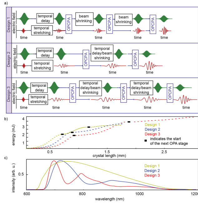
Figure 5. (a) Three designs are discussed in the main text. Design 1 consists of three OPCPA stages, where the residual pump energy after each amplification stage is reused in a subsequent OPCPA stage. Design 2 consists of two OPCPA stages. Here, the seed pulses are temporally stretched to twice the pump-pulse duration, and the residual pump energy after the first OPCPA stage is reused in the second stage. In Design 3, the seed pulses are temporally stretched to triple of the pump-pulse duration, and the residual of the pump energy is reused after each amplification stage. (b) Calculated amplified signal energy over the crystal length and their corresponding spectra (c) for the three different designs [7].
