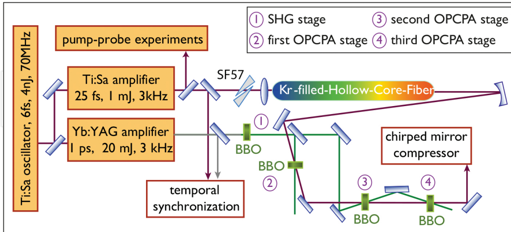
Figure 2. Block diagram of the OPCPA system. The OPCPA broadband seed pulses are generated from a Ti:Sa regenerative amplifier. The output of a Yb:YAG thin-disk amplifier, after frequency doubling, is used to pump the three OPCPA stages. Finally, a chirped-mirror compressor is used for pulse compression of the broadband amplified pulses.
