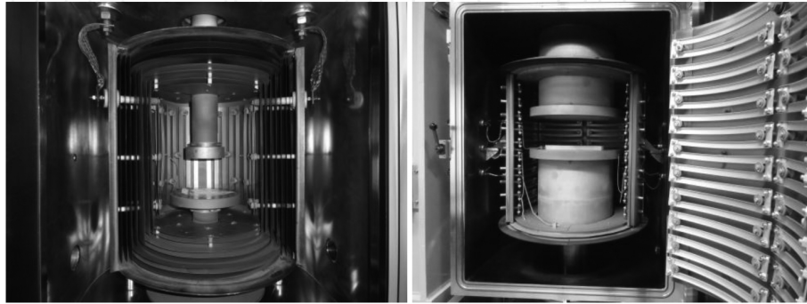
Figure 22. Diffusion bonding furnaces. Left: Maytec diffusion bonding furnace, maximum force 20 kN. Right: Systec diffusion bonding furnace, maximum force: 2 MN.
