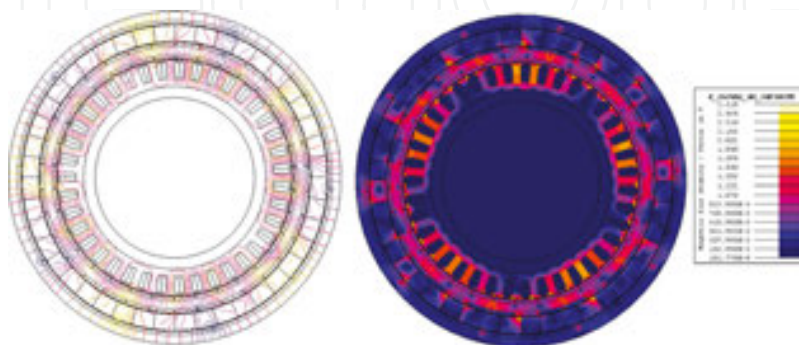
Figure 10. Integrated motor-gear analyzed variant, based on in-wheel motor: field lines (left) and flux density distribution (right) within the active parts.
