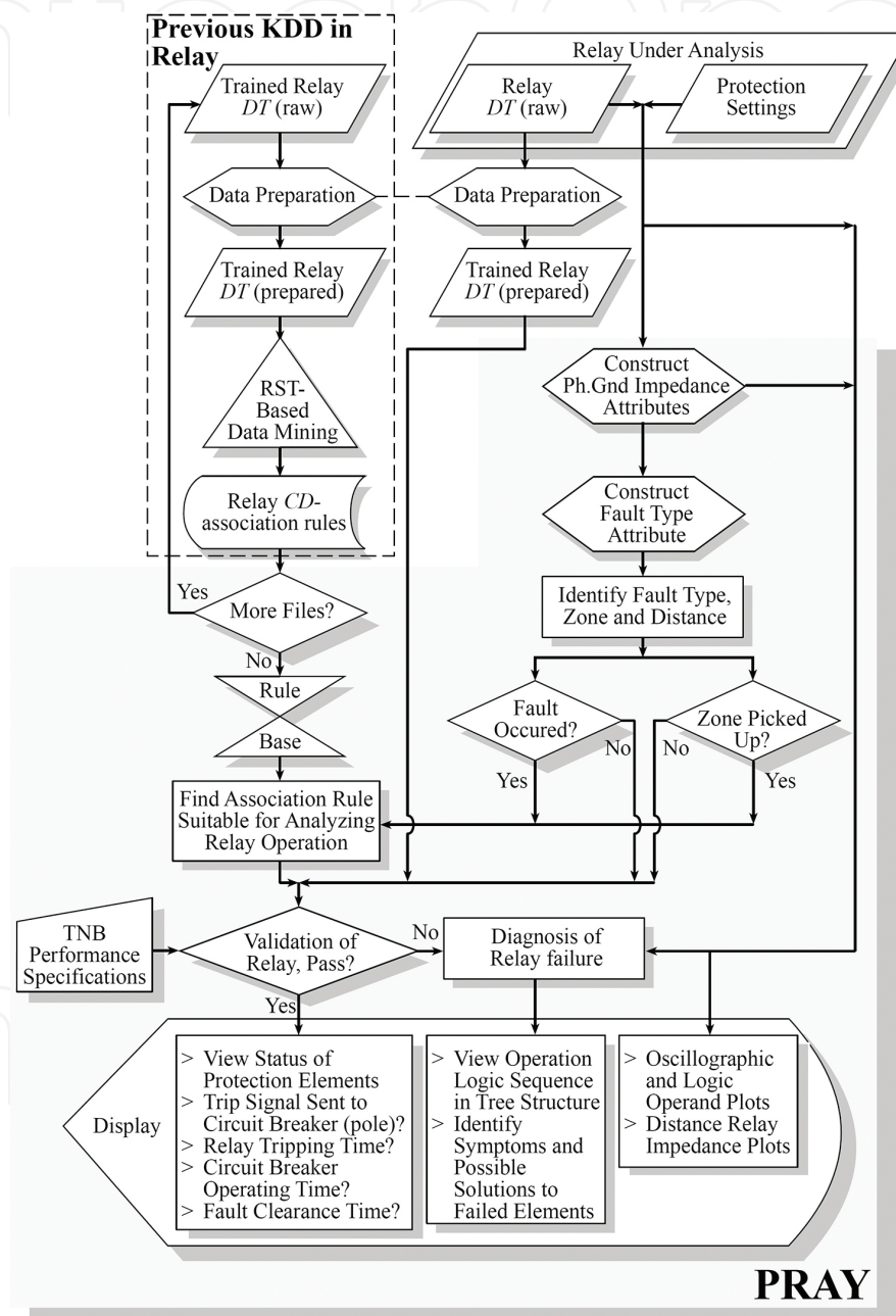
Figure 5. Architecture of Protective Relay Analysis System (PRAY).
