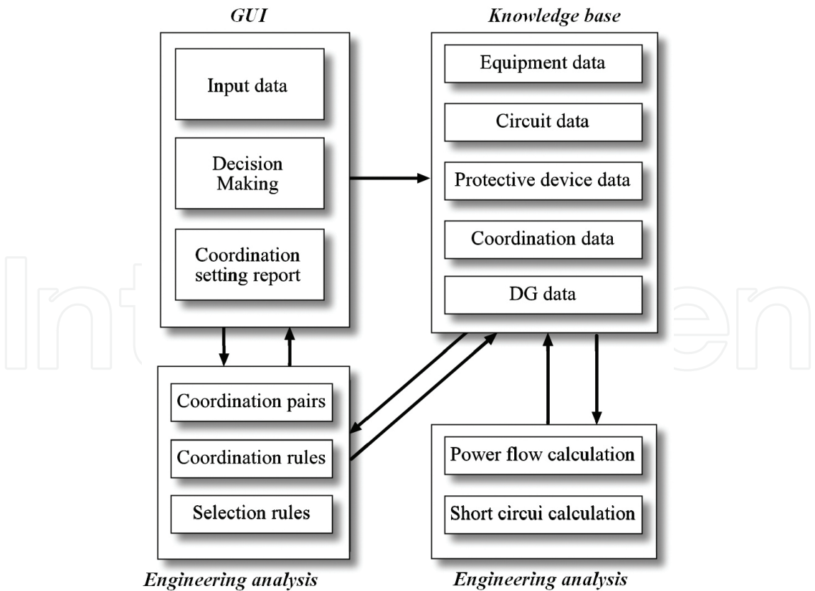
Figure 3. Structure of Expert System for protection coordination [13].
