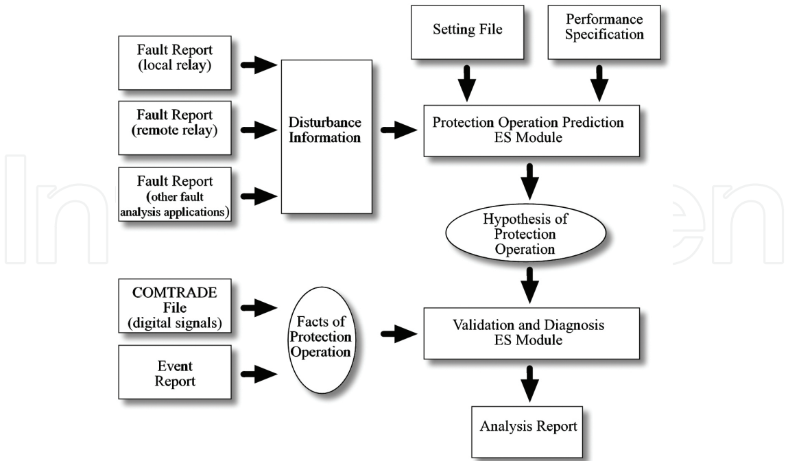
Figure 2. The Expert System block diagram for validation and diagnosis of protective relay [10].
