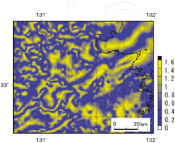
Figure 11. THETA map. Units are radians. This map indicates geological or structure boundary by line THETA = 0 .
