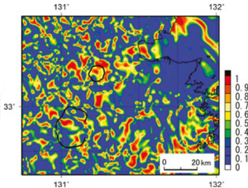
Figure 17. Map of dimensionality index, I . 2D structures are predicted in areas where I < 0.5 . Locations of the caldera rim are shown by black lines. The northern small caldera is the Shishimuta caldera and its diameter is 8–10 km. The southern large caldera is the Aso caldera and its diameter is approximately 25 km in the south-north direction and about 18 km in the east-west direction.
