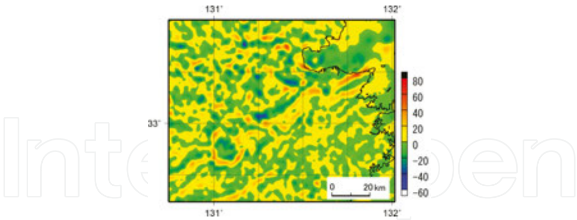
Figure 9. Vertical gravity gradient (second differential coefficient: \partial^2 g_z / \partial z^2 , g_{zzz} ) map. Units are given in E/km. E (Eötvös) is unit of the gravity gradient tensor, and 1 E = 0.1 mGal/km. This map indicates geological or structure boundary more sharply than g_{zz} .
