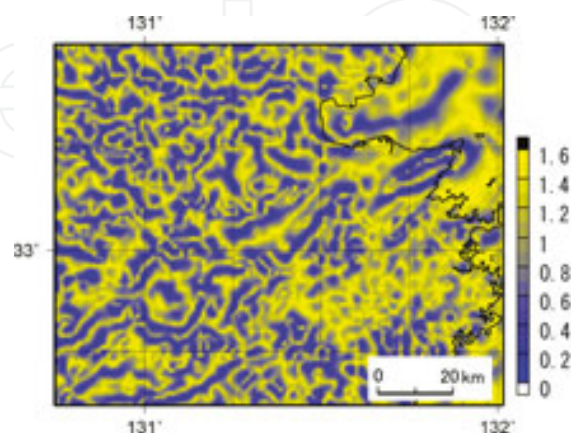
Figure 14. ILP map. Units are radians. This map extracts the edge of the gravity anomaly related to multi subsurface structures.
