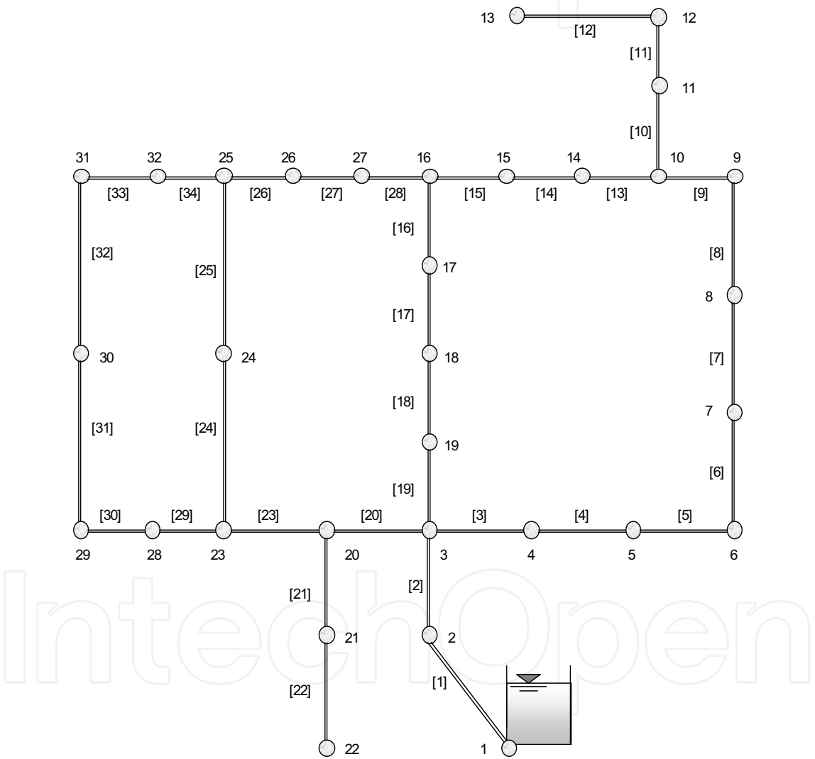
Figure 5. Network layout for the Hanoi Problem
