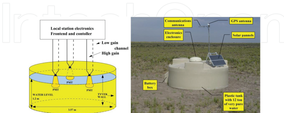
Figure 2. Water Cherenkov tank schematics. Each tank contains 12 tons of water as a radiator. The light is detected by three PMT, and each connected to a high- and a low-gain channel in the local station electronics.
