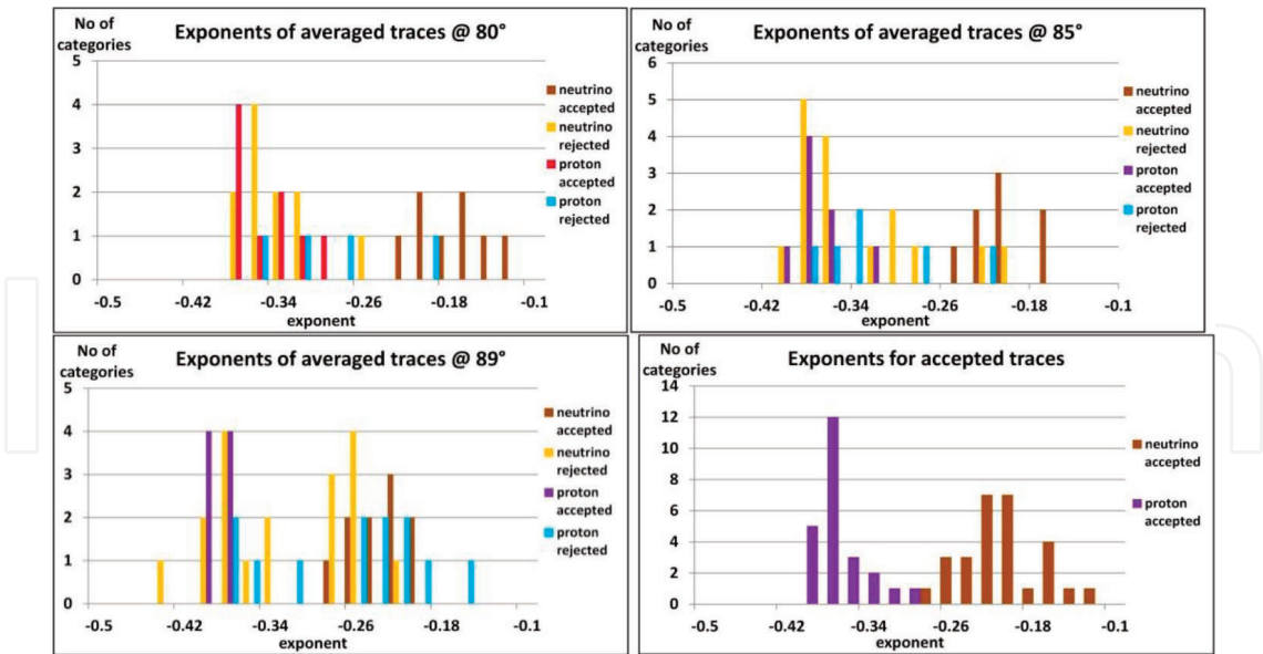
Figure 7. Histograms of exponents of rejected and accepted traces for protons and neutrinos. The accepted neutrino traces exponents are separated from the accepted proton traces exponents.
