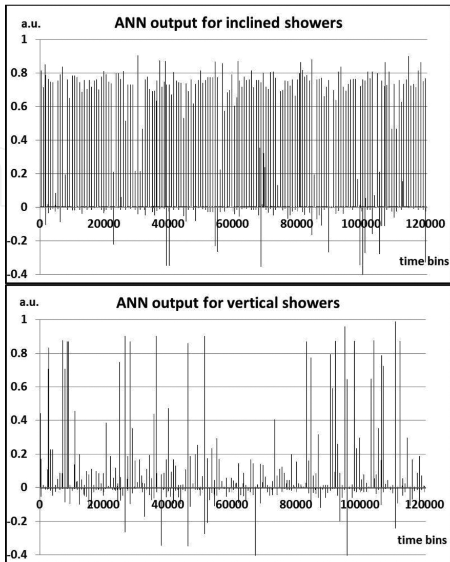
Figure 19. Graphs show the output of 12-8-1 neural network for positive-marked inclined showers (upper graph) and negative-marked vertical showers. Each graph shows 122,880 samples (768 samples/event). Outputs from the third neural layer are scaled to a range (-1, \dots, +1) .
