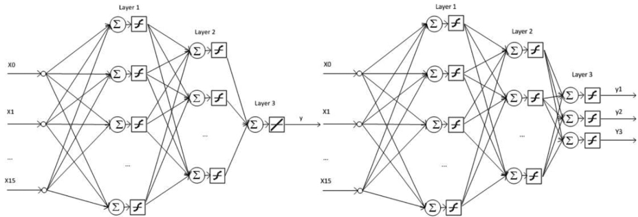
Figure 9. An internal structure of an FPGA neuron network with tansig function scaling output neuron data between consecutive layers. This right net contains more advanced last layer, which tries to separate patterns with higher efficiency.
