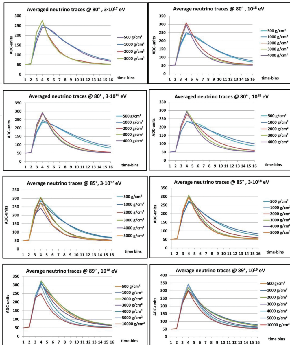
Figure 5. Plots contain averaged muon neutrino signal waveforms (ADC traces) for various angles, energies and initial-ization points. The exponents of the traces at distances 500 and 1000 g/cm 2 are different than on the rest of distances. This effect does not depend on the energy and slightly depend on the angle.
