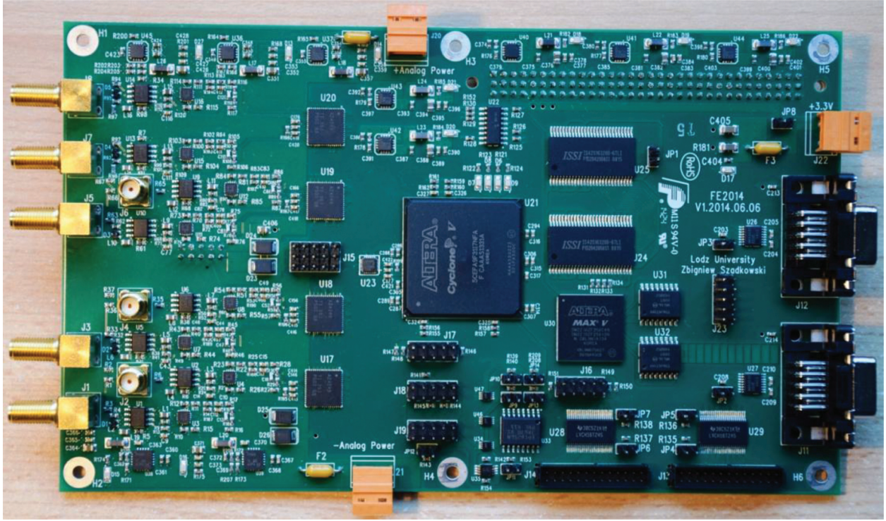
Figure 12. The front-end board with Cyclone V E FPGA used for high-resolution tests in the Pierre Auger Engineering Array.
