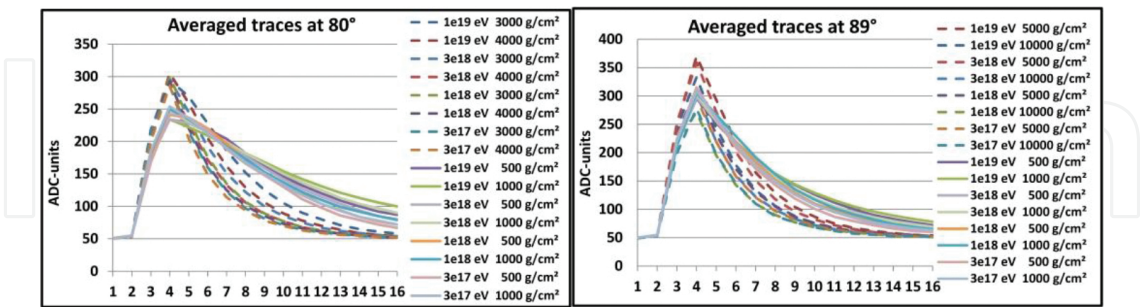
Figure 6. Plots show the differences between the traces produced by old proton showers (without markers) and young neutrino showers (with markers). Traces can be recognized on a base of exponential attenuation factors especially for relatively low angles (80°). Graphs show that for large zenith angles and very wide energy ranges, ‘old’ proton showers are attenuated faster than ‘young’ neutrino showers.
