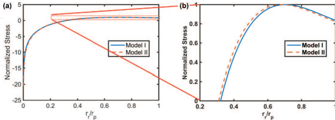
Figure 11. Normalized stress as a function of r_r/r_p (ring crack radius/plastic zone radius) predicted by the model I and model II (Poisson's ratio is assumed to be 0.21).
