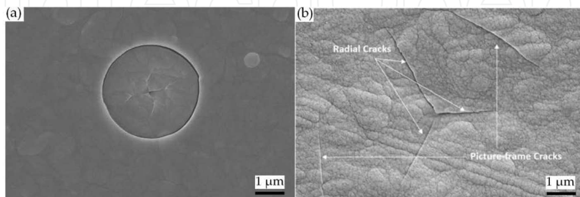
Figure 14. (a) Ring crack and (b) picture-frame crack [22] in a DLC film/PEEK substrate.
