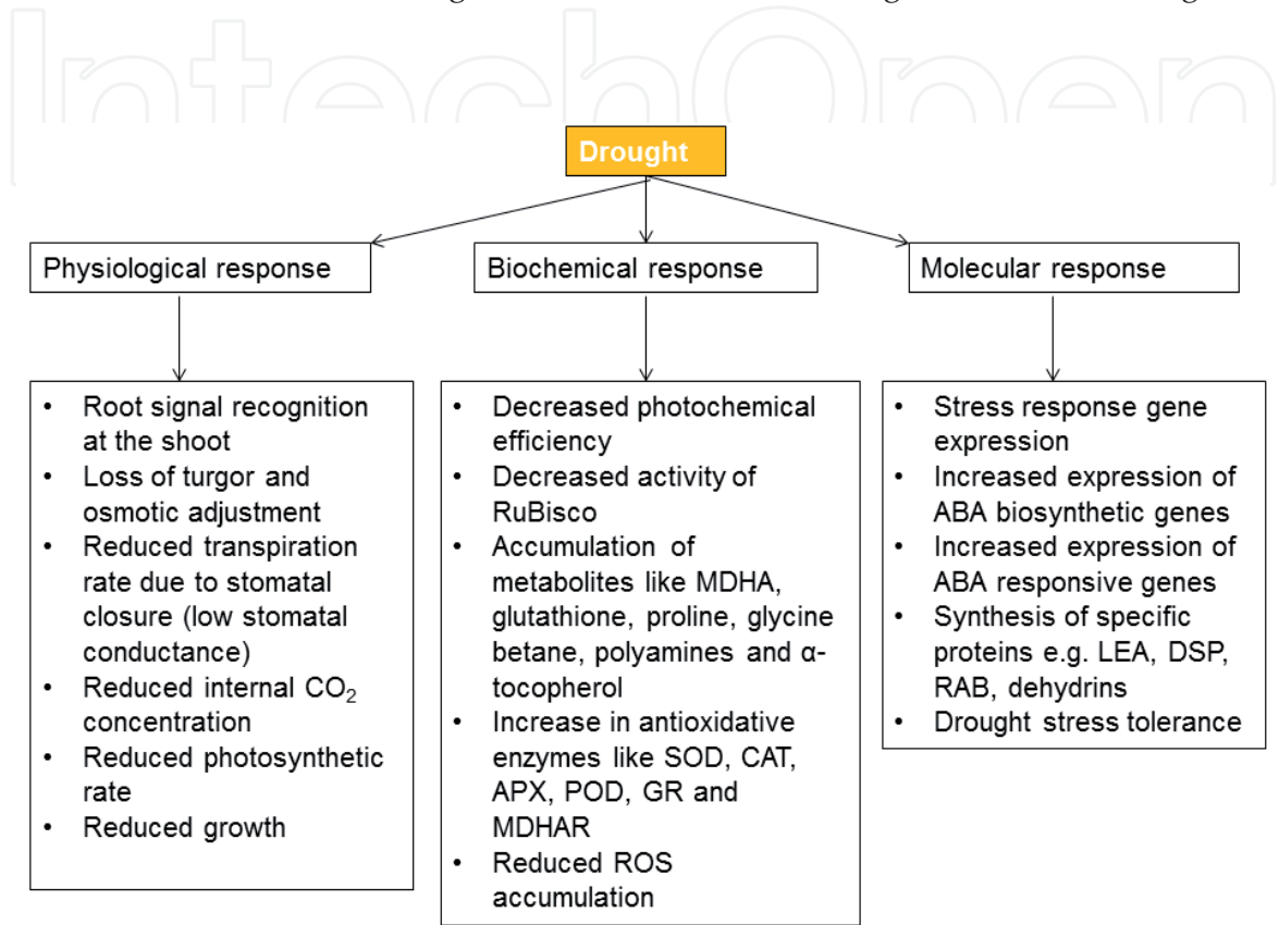
Figure 3. Physiological, biochemical, and molecular basis of drought stress tolerance in plants. Both major and minor changes that occur downstream of the transcriptional regulatory network are shown, although some of them, e.g. proline, glycine betaine and other amino acids, were previously shown not to be important in plant resistance to drought stress.
