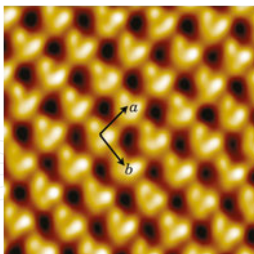
Figure 18. STM image of a single crystal of (EDO-TTF) 2 PF 6 in 4.7 \times 4.7 \text{ nm}^2 with the setpoint of 6.1 pA and the tip potential of 200 mV. Thermal drift was corrected with reference to the reported crystal structure [21] and FFT filter was applied. The assigned a and b axes are shown by the arrows.
