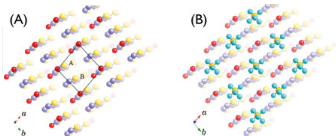
Figure 15. Structure of (EDO-TTF) 2 PF 6 at RT [21]. Crystal data are triclinic with a = 7.197 , b = 7.343 , c = 11.948 Å, \alpha = 93.454^\circ , \beta = 75.158^\circ , \gamma = 97.405^\circ . Blue, yellow, and red balls indicate carbon, sulfur, and oxygen atoms, respectively. Hydrogen atoms are not indicated. The unit cell contains two EDO-TTF molecules and one PF 6 - ion. (B) shows relative location of PF 6 - ions to EDO-TTF molecules.
