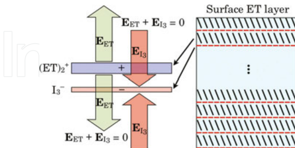
Figure 1. Schematic picture of the electric field produced by a (\text{ET})_2^+ and \text{I}_3^- double layer with the same total charges of each layer in \alpha\text{-(BEDT-TTF)}_2\text{I}_3 . The electric field of the double layer is confined inside the double layer. That is, outside the double layer, the electric field cancels out. However, the leakage electric field near the double layer forms the electric dipolar field, which binds the neighboring double layers. Thus, the surface ET layer approximately feels only the electric field of the \text{I}_3^- layer within the double layer (reused from Ref. [1]).
