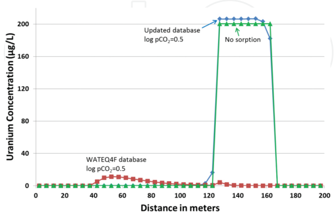
Figure 12. Uranium concentrations in groundwater at 25 years with 500 ppm Fe and CO 2 in recovery zone of log pCO 2 = 0.5 and infinite calcite down-gradient. The triangles show no sorption, the diamonds show the updated database, and the squares show the Wateq4f database.
