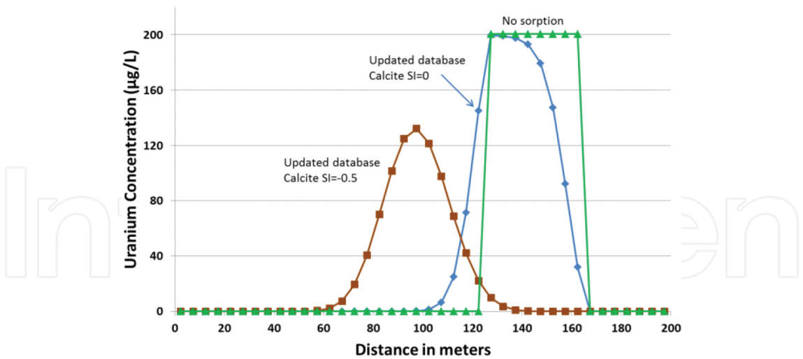
Figure 10. Uranium concentrations in groundwater at 25 years with 500 ppm Fe. The triangles show no sorption, the diamonds show the updated database, and calcite saturation index set to 0.0. The squares show the updated database, and calcite saturation index set to -0.5.
