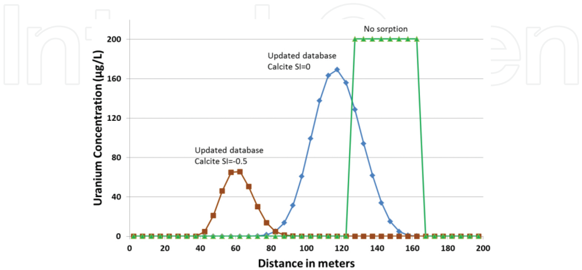
Figure 9. Uranium concentrations in groundwater at 25 years with 2500 ppm Fe. The triangles show no sorption, the diamonds show the updated database, and calcite saturation index set to 0.0. The squares show the updated database, and calcite saturation index set to -0.5.
