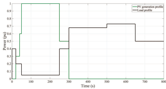
Figure 7. Load and generation profiles at each bus.
