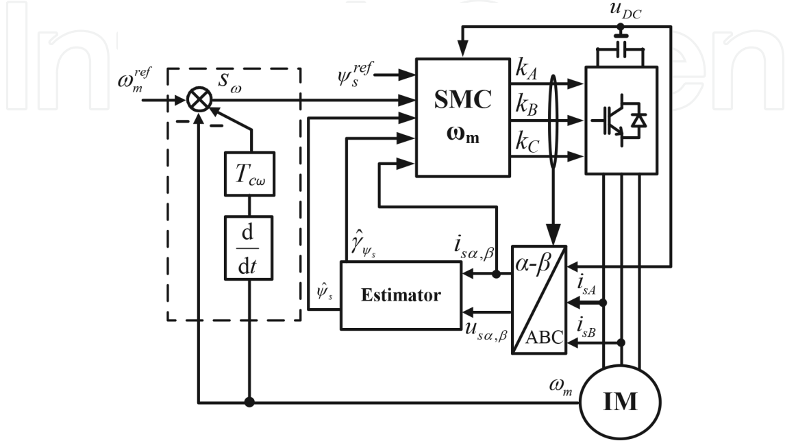
Figure 4. Block diagram of the direct SM speed control.
