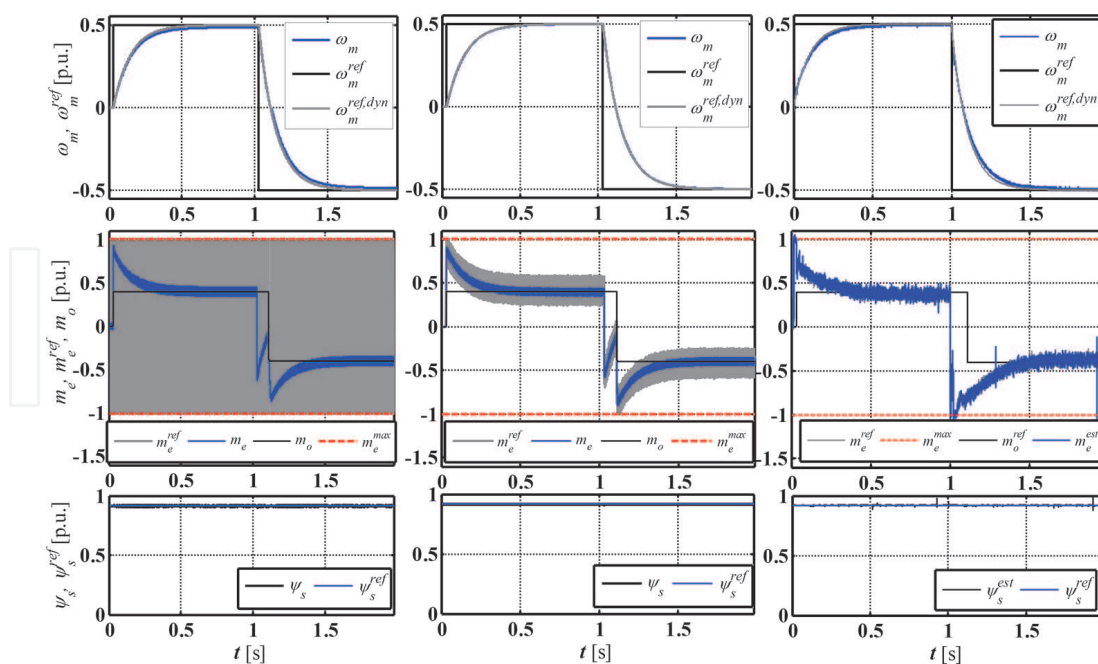
Figure 7. Performance of the SM cascade speed control: (a) simulation study: relay control, (b) simulation study: equivalent control, (c) experimental study: equivalent signal-based control; first row: reference and real speed, second row: load, electromagnetic and maximum torques, third row: reference and real amplitude of stator flux.
