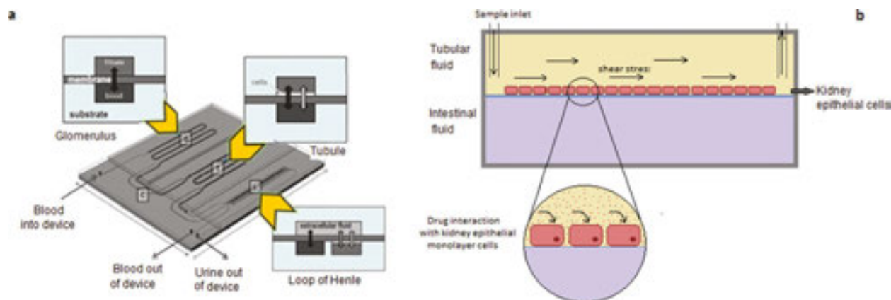
Figure 12. (a) Nephron on a chip: Schematic of the chip with cross sections of three functional units named glomerulus, proximal convoluted tubule and loop of Henle, which are responsible for filtration, reabsorption and urea concentration, respectively. (b) Kidney reabsorption functions using a microfluidic chip comprising of an apical channel separated from a bottom channel by proximal tubular epithelial cells cultured ECM-coated porous membrane [94].
