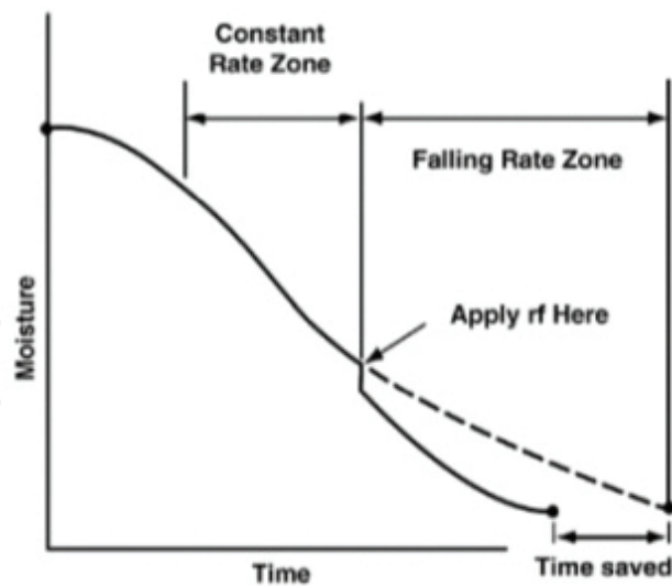
Figure 11. Effect of microwave drying on normal drying curve [75].
