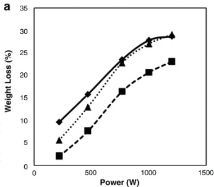
Figure 12. Effect of microwave power level on coal weight loss for three different coal types [5].
