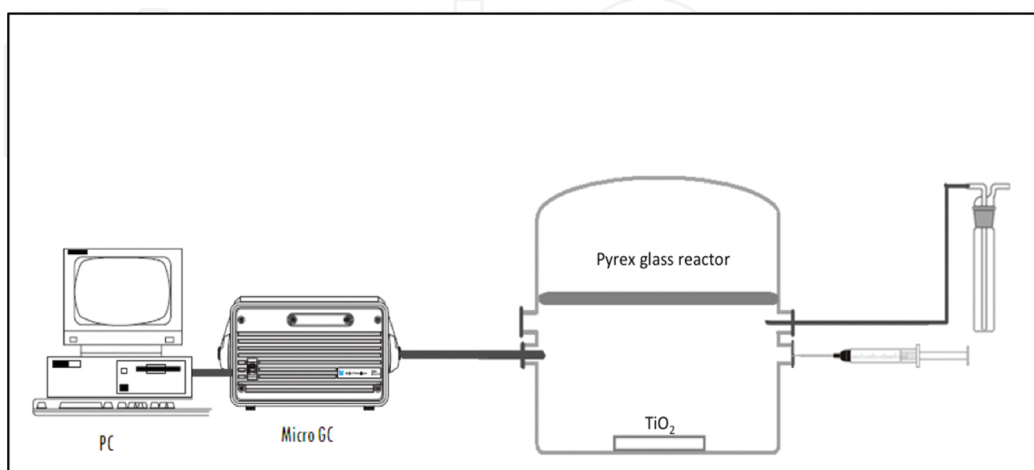
Figure 2. VOC photodegradation—set-up.
