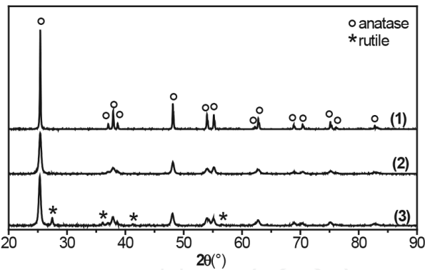
Figure 5. XRD patterns of K1077 (1), PC105 (2) and P25 (3).
