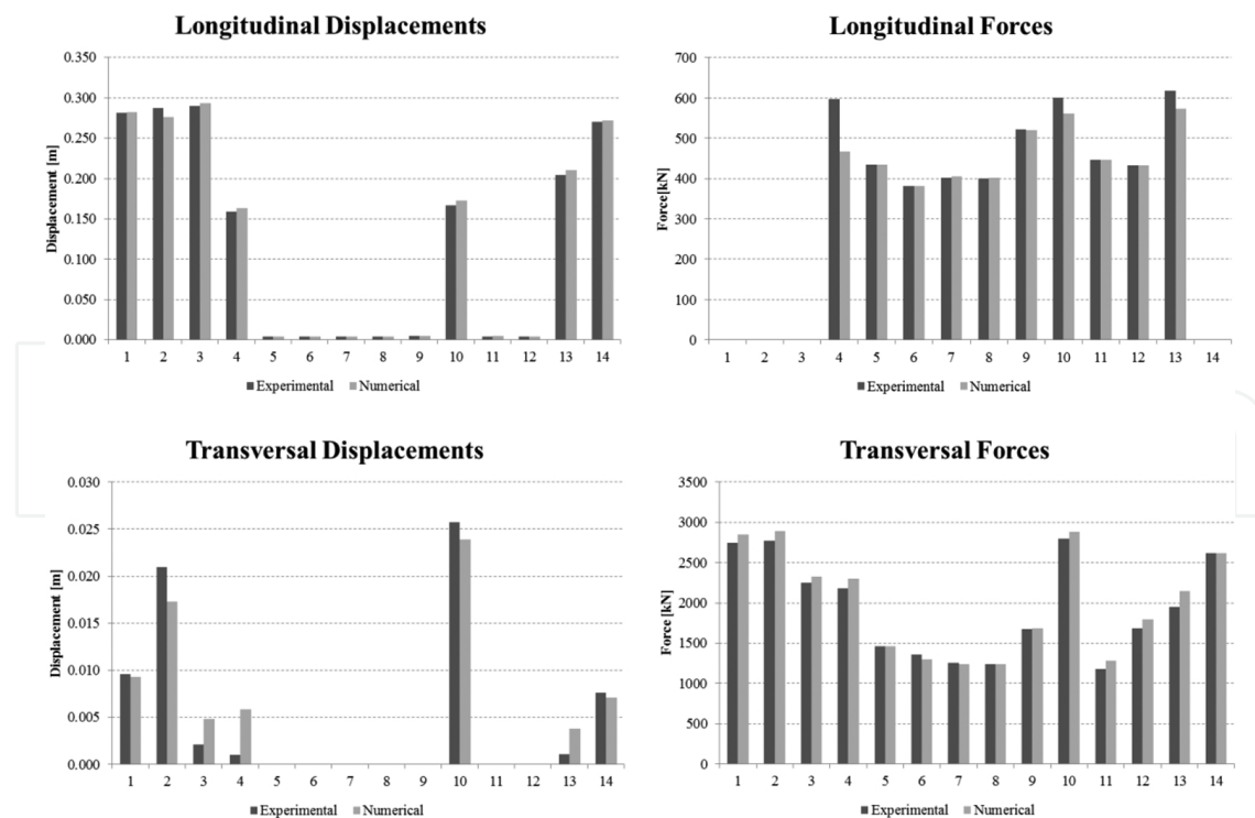
Figure 11. Bar charts representing forces and displacements on the level of the devices—comparison between experimental and numerical results.
