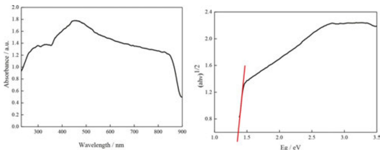
Figure 28. (a) UV-Vis diffuse reflection spectra of yolk-shell \text{TiO}_x\text{N}_y/\text{TiN} . (b) The plots of (\alpha h\nu)^{1/2} versus h\nu . The band gap of yolk-shell \text{TiO}_x\text{N}_y/\text{TiN} .
