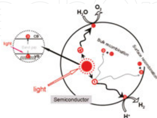
Figure 4. Processes in photocatalytic water splitting. Reprinted with permission from ref [15]. Copyright 1995 American Chemical Society.
