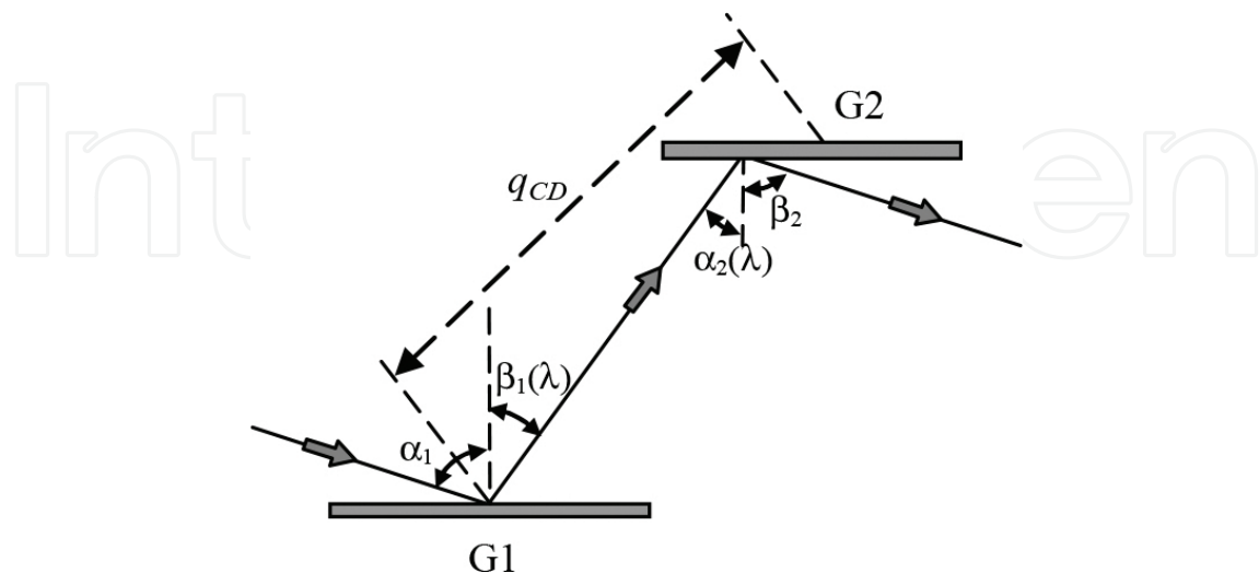
Figure 3. Double-grating compressor in the CDG. The diffraction angle from G2 is constant with the wavelength and equal to the incidence angle on G1, \beta_2 = \alpha_1 .
