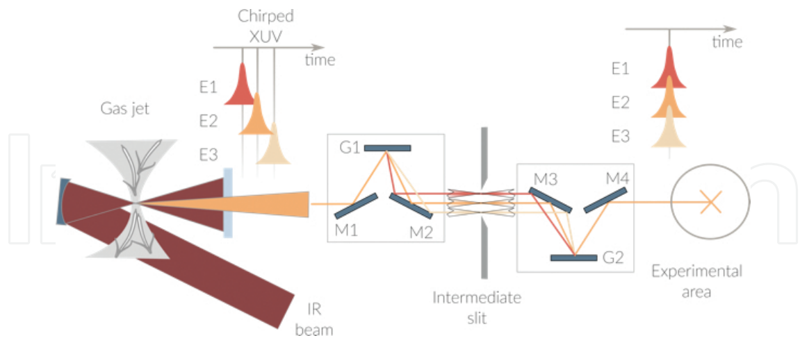
Figure 15. Schematic of the attosecond compressor.
