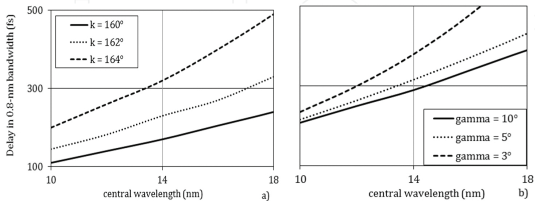
Figure 7. Delay in 0.8-nm bandwidth introduced by the compressor having the parameters of Table 2 when the gratings are rotated to tune the wavelength in the 10–18 nm interval: (a) CDG, variable subtended angle; (b) OPG, variable altitude angle.
