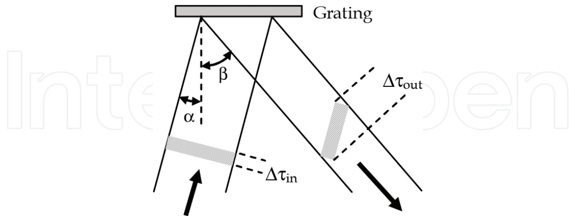
Figure 2. Pulse-front tilt of an ultrashort pulse diffracted by a grating in the CDG. \Delta\tau_{in} and \Delta\tau_{out} are the pulse duration at input and output, respectively. At the first diffracted order, the pulse-front tilt is \Delta OP = N\lambda , where N is the number of illuminated grooves.
